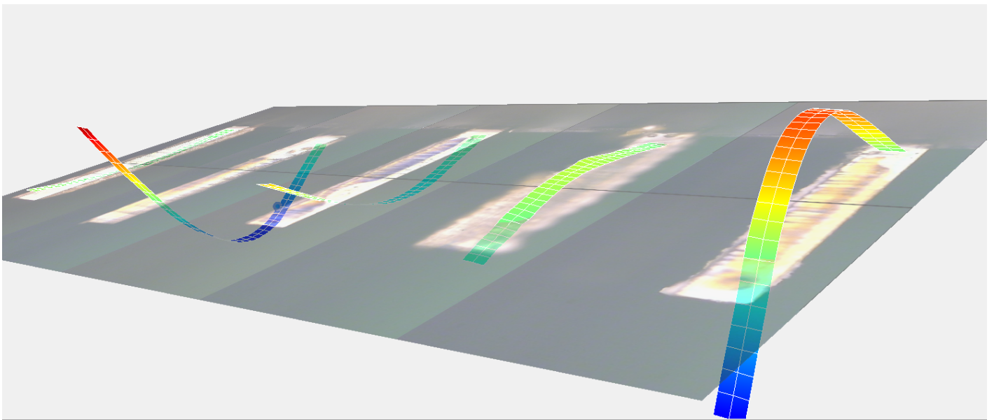
Figure 4.6: 2nd Bending mode with the 5 beams
