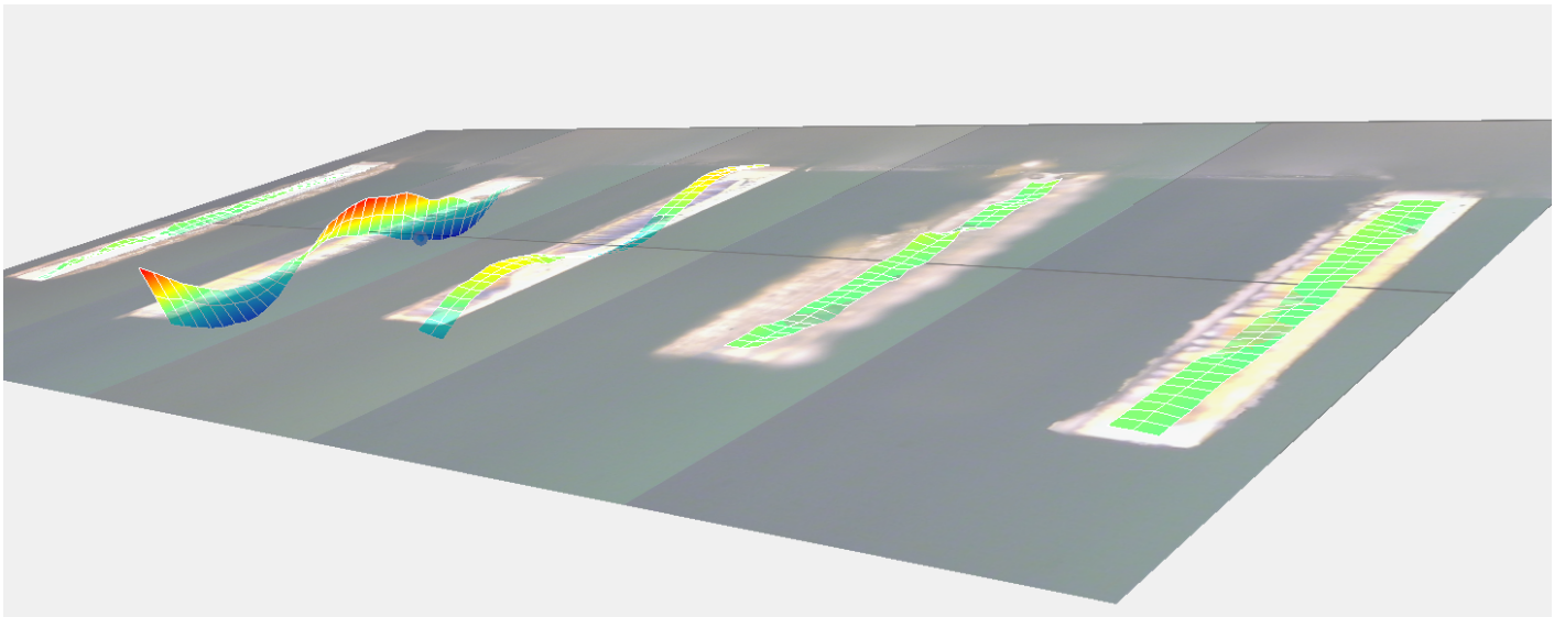
Figure 4.10: Using the devices with 5 beams, the 2nd beam shows the 3rd Torsion mode
