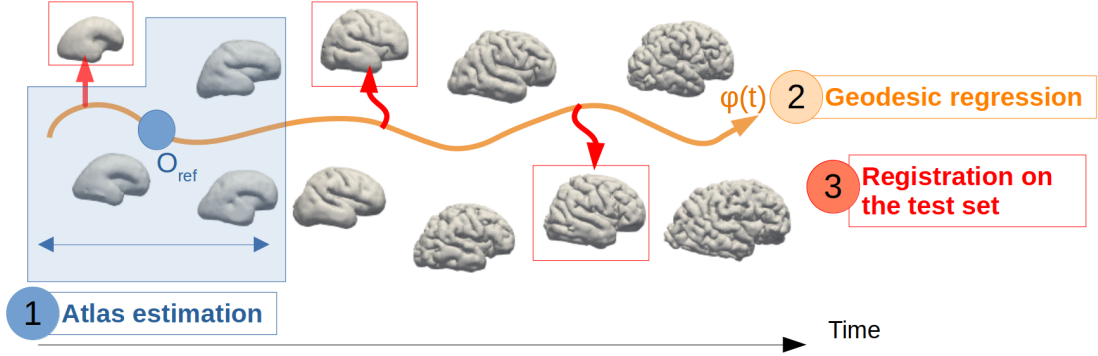
Figure 4.5: Three-step evaluation procedure illustrated on the dataset of cortical surface meshes. Cortices outlined in red belong to the test set. O_{ref} : template object estimated during step (1). \phi(t) : (piecewise) geodesic trajectory estimated during step (2).
