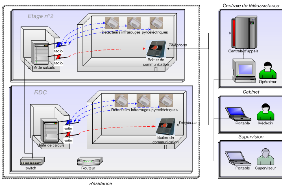
Figure 64 : Architecture matérielle.
