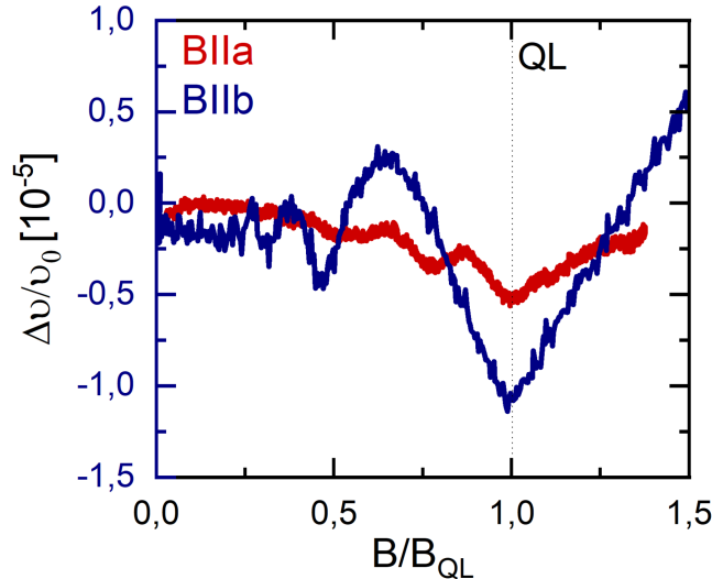
Figure 8.2: Ultrasound attenuations in \text{ZrTe}_5 : Sound-velocity variation \Delta v/v_0 of a longitudinal sound mode propagating along the a -axis as a function of magnetic field applied along the a -axis (red) and b -axis (blue) at 1.7 K. For clarity the magnetic field in both measurements is scaled with respect to the quantum limit ( B_{QL}^a = 12\text{T} and B_{QL}^b = 1.2\text{T} ). The change of the sound velocity corresponds to the change of the phonon contribution to the thermal conductivity with B .
