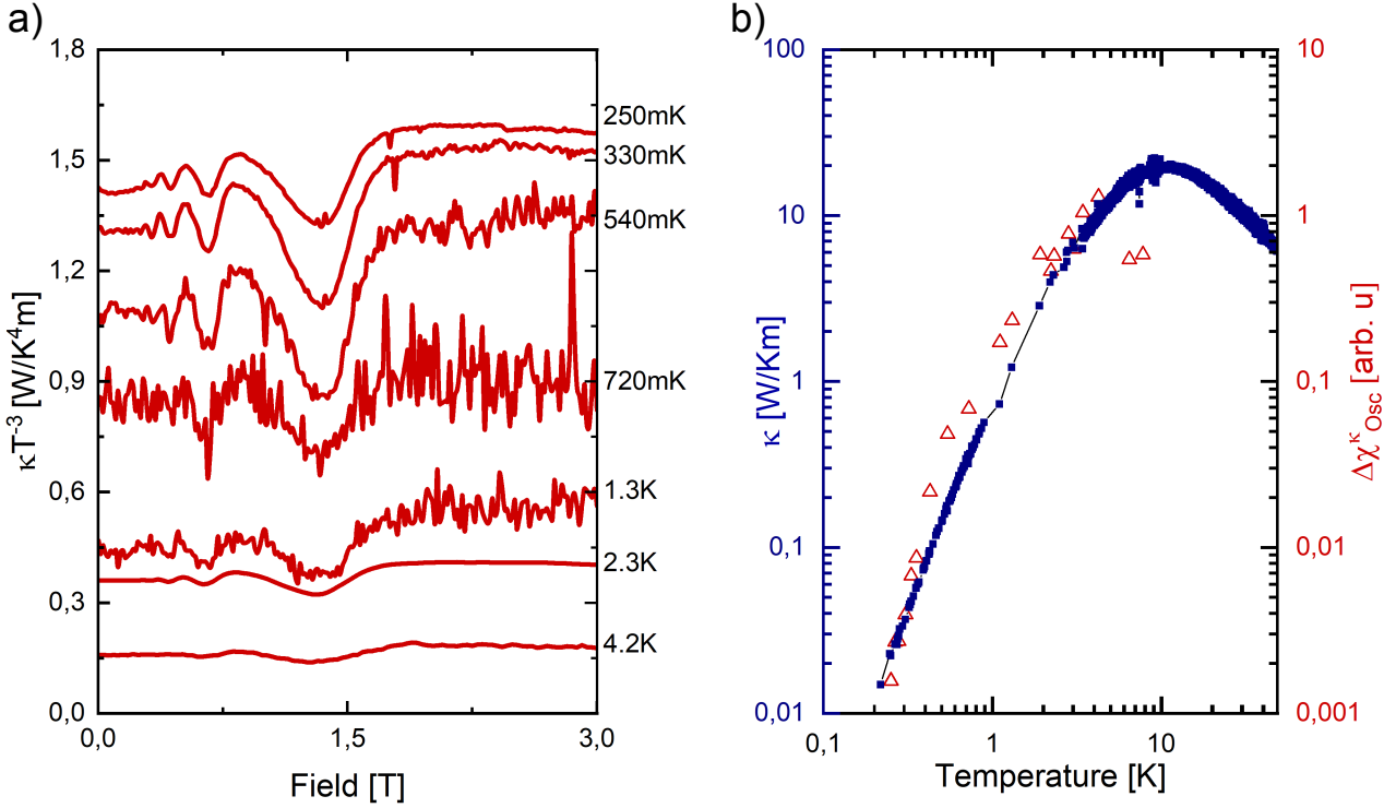
Figure 8.9: Temperature dependance of the magnetothermal quantum oscillation amplitude in \text{ZrTe}_5 . a) Example traces of magnetothermal conductivity divided by T^3 for clarity of presentation. b) Comparison of the temperature dependence of zero field thermal conductivity with the temperature dependence of the amplitude of the last oscillation. (red).
