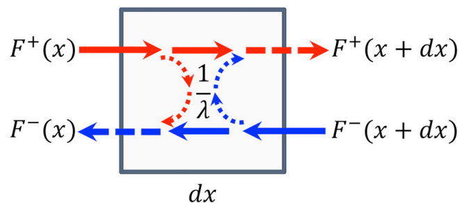
Figure 5.2: Scheme of the scattering process considered
