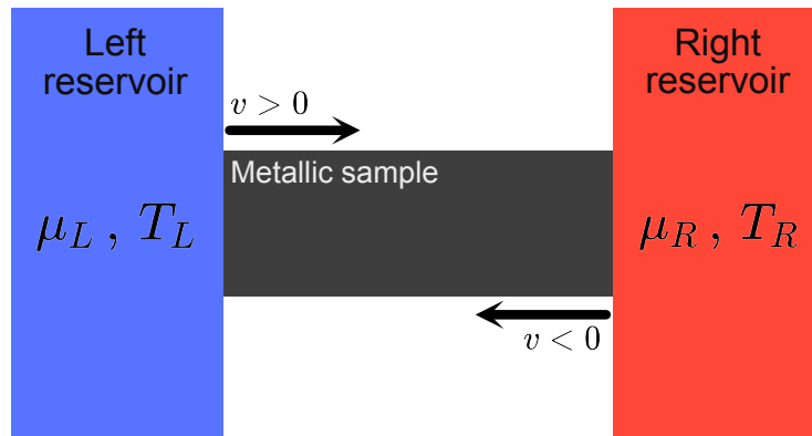
Figure 8.6: Chiral notations Right-movers, defined by their positive velocity ( v > 0 ), come from the left reservoir and possess a chemical potential \mu_L and a temperature T_L . Similarly, left movers, defined by their negative velocity ( v < 0 ), come from the right reservoir and possess a chemical potential \mu_R and a temperature T_R .
