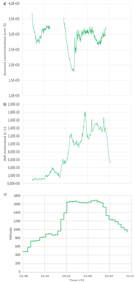
Figure 2.24: As in Figure 2.15 but for the OO case and only for a) total aerosol particle number concentration ( N_{AP,OO} ), b) INP concentration ( N_{INP,OO} ) derived from the parameterisation of DeMott et al. (2010) and c) flight altitudes for Polar 6 aircraft.
