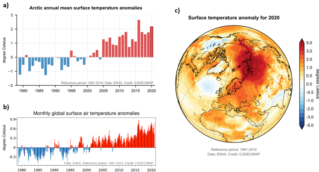
Figure 1.7: Time series of (a) Arctic annual mean surface temperature anomalies (averaged over 66.6^{\circ}\text{N} - 90^{\circ}\text{N} ) and of (b) monthly global-mean surface air temperature anomalies, both from 1979 to 2020. (c) Map of the annual mean surface temperature anomaly in 2020. All anomalies are calculated relative to the 1981-2010 mean. Figure adapted from ESOTC (2020).
