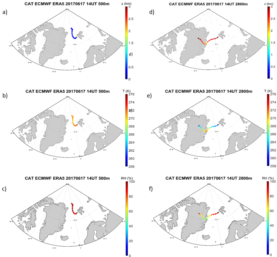
Figure 2.23: As in Figure 2.14 but for the two cloud layers of the OO case.
