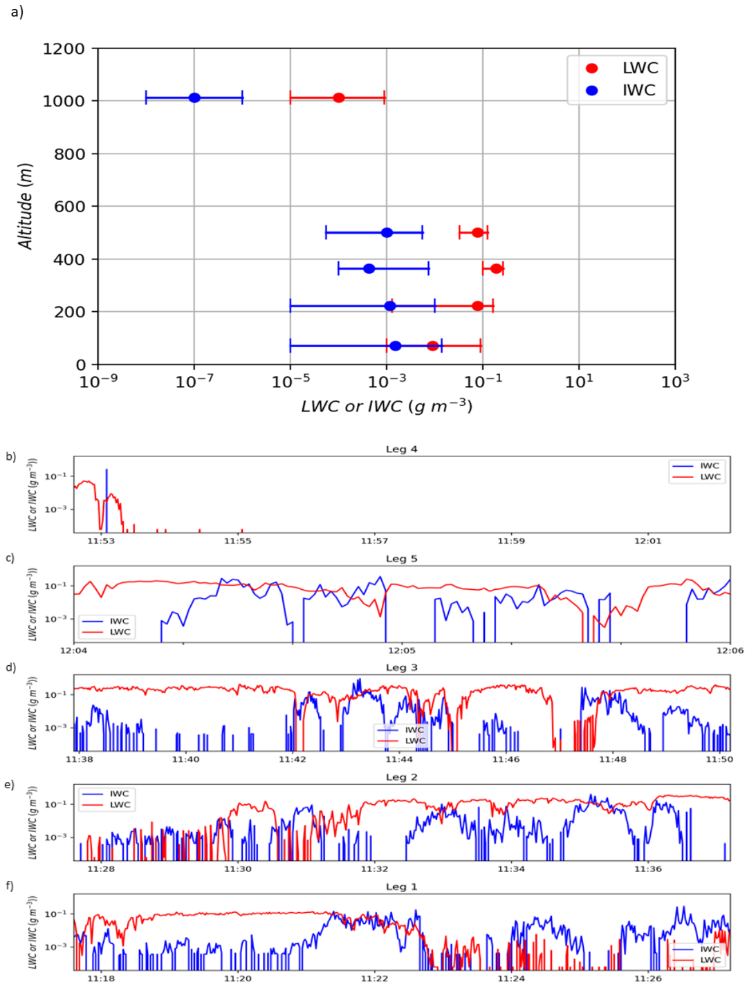
Figure 2.20: a) Vertical profile of the liquid ( LWC ) and ice water ( IWC ) contents for the SI case from CPI and CDP measurements. Points correspond to the median of the observed data (for the different legs) and intervals indicate the first (Q1) and the third (Q3) quartiles. b-f) Temporal evolution of ( LWC ) and ice particles ( IWC ) for each leg (see Figure 2.8a for corresponding altitudes). Each parameter characterising the liquid or the ice phase are plotted in red or in blue, respectively.
