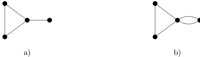
Figure 2.1: Graphs a) and b) both fulfill the criteria of being quasi-bipartite according to our definition. However, when considering the definition provided by Ding et al. [27], only graph a) conforms, while graph b) does not meet their criteria for quasi-bipartiteness.
