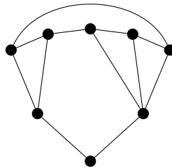
Figure 1.8: A near-brick having two vertex-disjoint odd cycle and whose only brick is W_5 which is odd intercytic.
