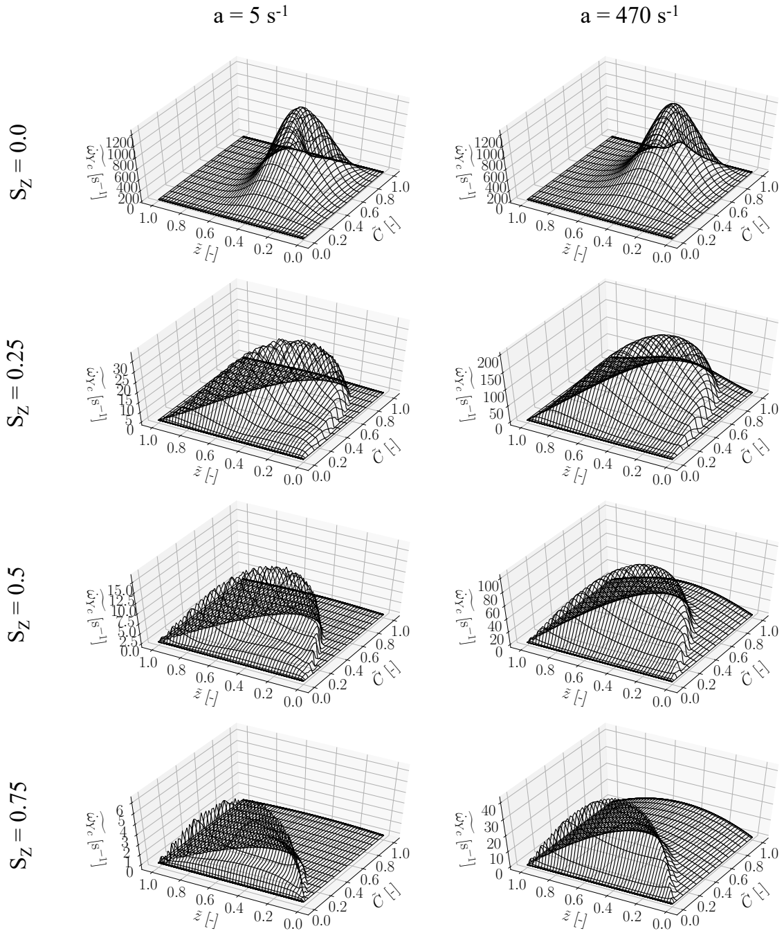
Figure B.9: Slices of the filtered progress variable source term \widetilde{\dot{\omega}}_{Y_c} as a function of the filtered mixture fraction \tilde{z} and of the filtered normalized progress variable \tilde{C} , for different strain rates a and different mixture fraction segregation values S_z . Note the evolution of the vertical scale
