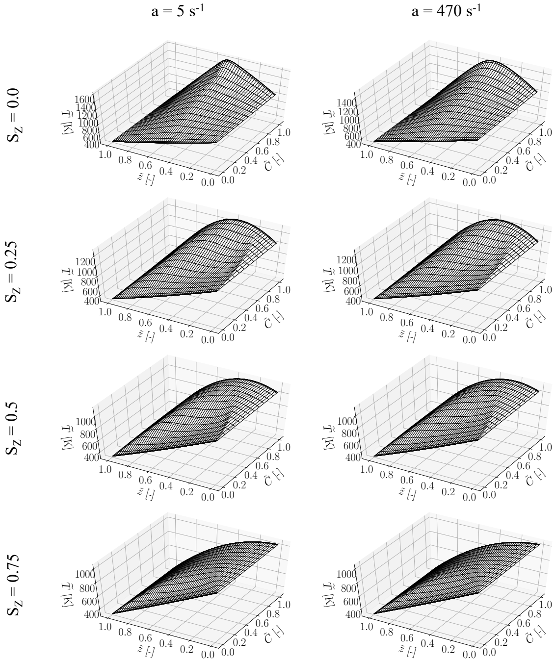
Figure B.7: Slices of the filtered temperature \tilde{T} as a function of the filtered mixture fraction \tilde{z} and of the filtered normalized progress variable \tilde{C} , for different strain rates a and different mixture fraction segregation values S_z
