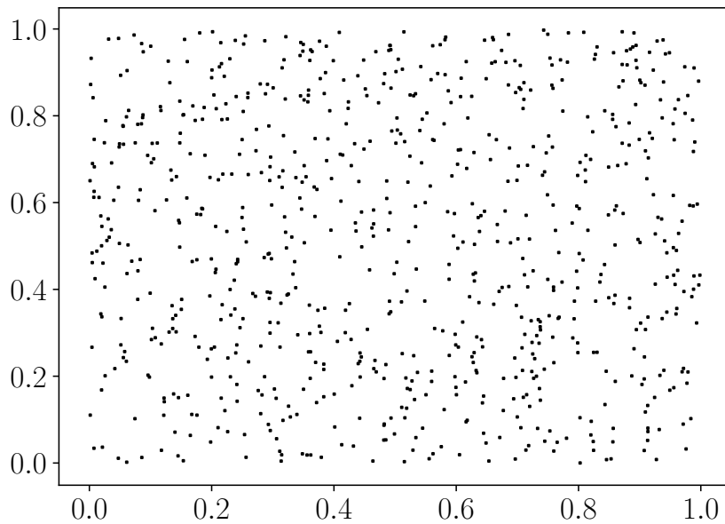
Figure 1.1: 800 points of a Monte-Carlo sampling of a 2D uniform random vector on the unit hypercube
