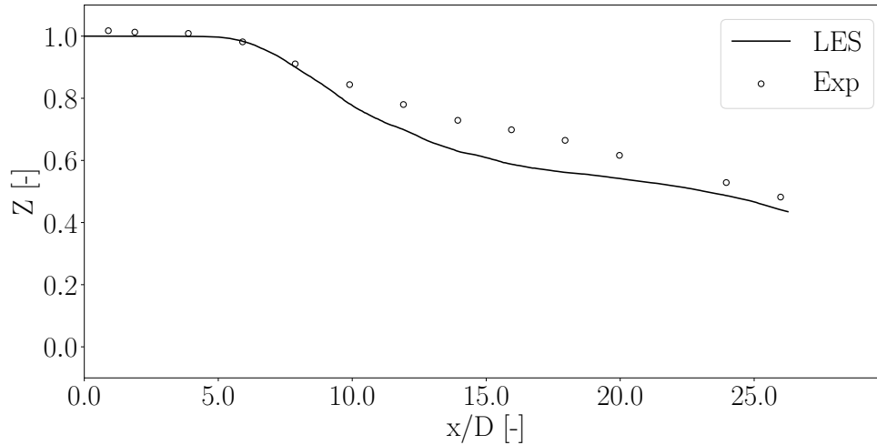
Figure 3.12: Axial profile of the mixture fraction Z in the LES, compared to the measurements from [11]
