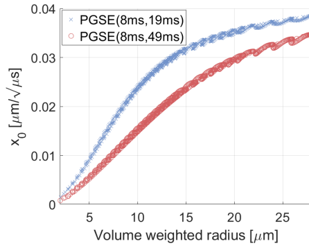
Figure 4.19: x_0 against the volume-averaged soma radius for two spheres case. Each scatter point represents one combination of (R_1, R_2) \in [2, 28]^2 . The blue and red scatters represent the results using the short and long sequences.
