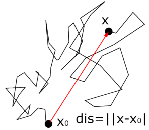
Figure 1.8: Isotropic diffusion process in an unbounded medium. Particles can move freely in the medium.
