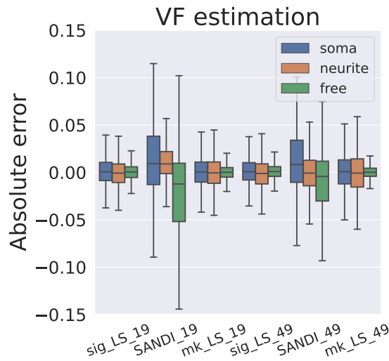
Figure 4.23: The box plots summarizing the distributions of the absolute errors of f_{\text{soma}} , f_{\text{neurite}} , f_{\text{free}} . The estimations are computed by (1) Synthetic library search based on signals, (2) SANDI library search, and (3) Synthetic library search based on IP-derived biomarkers on the Synthetic test set. The Synthetic voxels set has 1.45 million artificial voxels containing neurons and a free diffusion compartment. The Synthetic test set has 450,000 voxels from the Synthetic voxels set. A box plot denotes the median, interquartile range, and 1.5 times the interquartile range by the center line, hinges, and whiskers.
