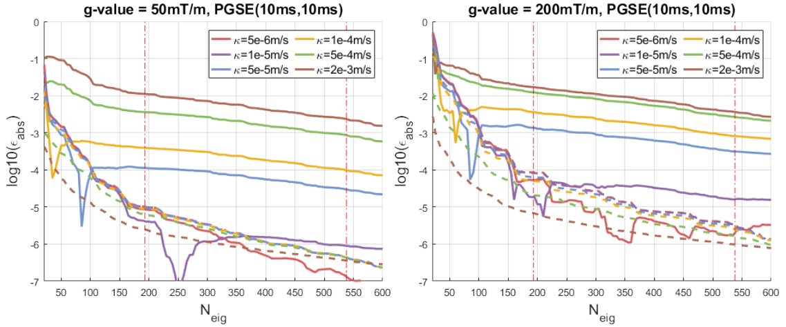
Figure 2.4: Normalized signal errors of the new method (in solid line) and the Numerical Matrix Formalism method (in dashed line), compared to the reference solution, as a function of N_{eig} . The two vertical lines indicate where the truncations occur for L_s = 2\mu\text{m} ( N_{eig} = 193 ) and L_s = 1\mu\text{m} ( N_{eig} = 538 ). The simulations are performed on \Omega^I , with gradient direction fixed in [\sqrt{2}/2, \sqrt{2}/2, 0]^T and the sequence PGSE(10ms, 10ms). Left: g -value= 50 mT/m; Right: g -value= 200 mT/m.
