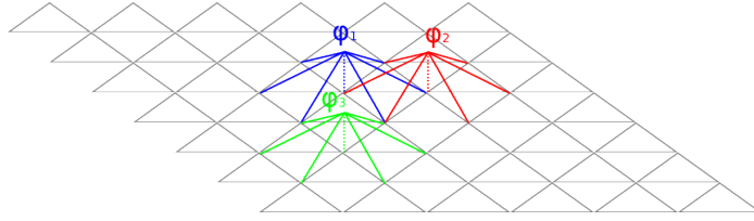
Figure 1.17: P1 linear function \varphi defined on a discretized domain \{\mathcal{T}^h\} in two-dimensional space.
