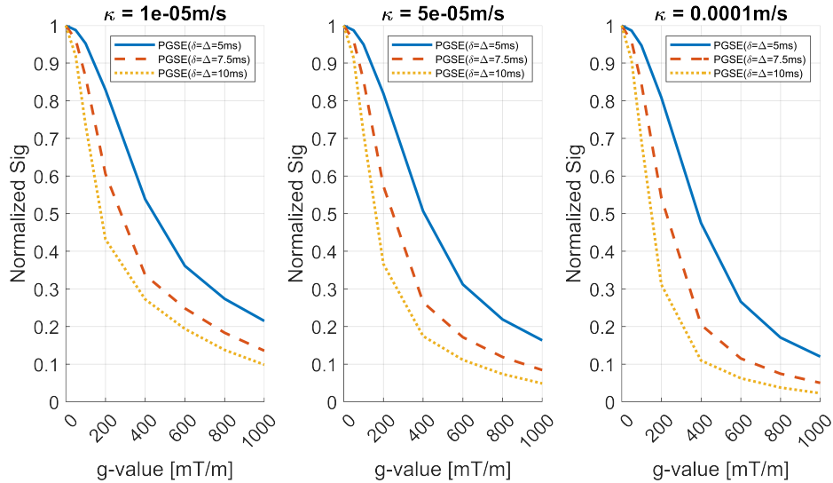
Figure 2.2: Normalized direction-averaged diffusion MRI signals as a function of the g -value \|\mathbf{g}\| . These are the reference solutions computed using the Numerical Matrix Formalism method with the full set of permeable Laplace eigenfunctions, i.e., N_{eig} = N_{node} = 3455 eigenfunctions for \Omega^I .
