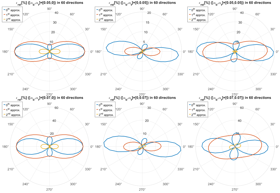
Figure 3.4: The relative ADC error between 0^{th} , 1^{st} and 2^{nd} order approximations and the reference value in 60 gradient directions, which are uniformly distributed in the x-z plane ( y = 0 ). The labeled values on the gray circles are given in percent. The gradient sequence is PGSE(5ms, 15ms). The displayed angle (from 0 to 360 degrees) is the angle between positive x-axis and the diffusion gradient direction. The blue, red, yellow lines represent 0^{th} , 1^{st} and 2^{nd} order approximations, respectively. Top left: \alpha_b = 0.05 ; Top middle: \alpha_t = 0.05 ; Top right: [\alpha_b, \alpha_t] = [0.05, 0.05] Bottom left: \alpha_b = 0.07 ; Bottom middle: \alpha_t = 0.07 ; Bottom right: [\alpha_b, \alpha_t] = [0.07, 0.07] .
