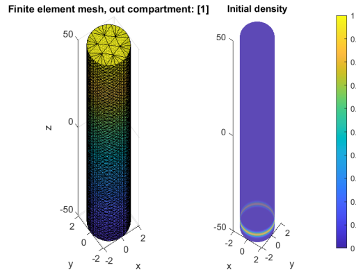
Figure 5.2: Left: Finite elements mesh of the simulation domain \Omega , with a radius of 2.1\mu\text{m} and a height of 100\mu\text{m} . Right: The initial density on \Omega . We adjusted the plot z-coordinate scale to enhance its visual representation.
