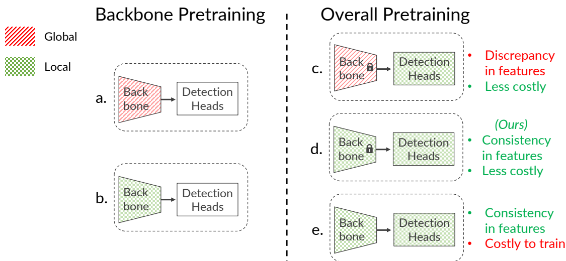
Figure 5.2. Illustration of the different pretraining possibilities for Object Detection. The pretraining can be either limited to the backbone (left), or overall including the detection heads (right). The few previous overall approaches either suffer from a discrepancy in the features between the backbone, that is trained at the image-level (global), and the detection heads, trained to encode object-level (local) information (c.), or from the cost of training lots of parameters with a large batch size (e.).
