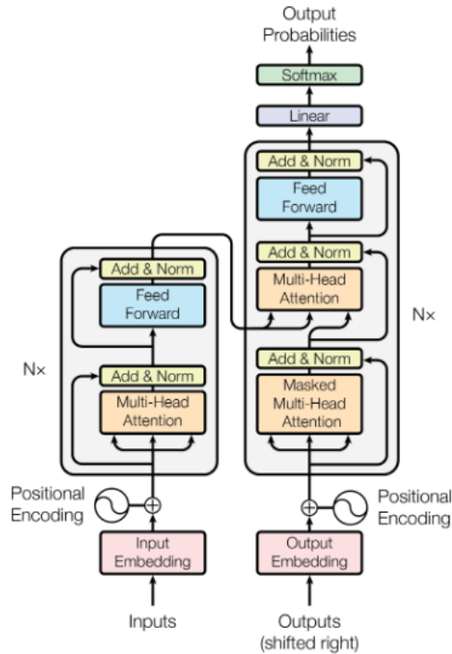
Figure 2.8. The Transformer encoder-decoder architecture from [Vaswani et al., 2017] used for NLP tasks. The left and right halves respectively represent the Transformer encoder and Transformer decoder architectures.
