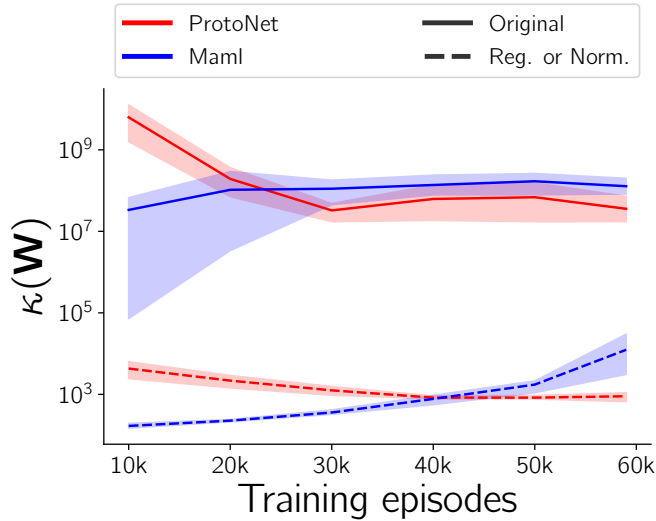
Figure 4.7. Evolution of \kappa(\mathbf{W}) on 5-way 1-shot episodes from minilmageNet, for ProtoNet (red, straight lines), MAML (blue, straight lines) along with their regularized and normalized counterparts (respectively the same colors, in dashed lines).
