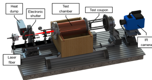
Figure 1.4. – BLADE laser bench of the ONERA (Leplat et al., 2016)
