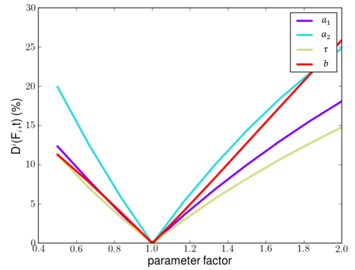
Figure 3.9. – Influence of parameter values on D^i(F_i, t) according to time at 600°C
