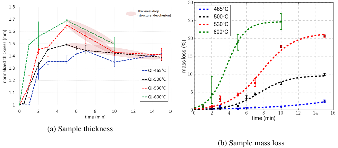
Figure 3.5. – Evolution over time of the geometry-based method characteristic quantities (thickness and mass) in QI laminates for different temperatures of exposure
