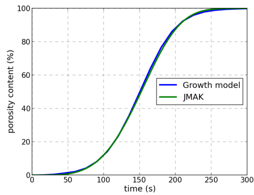
Figure 3.25. – Comparison of the porosity content evolution over time as obtained by the JMAK model and the nucleation-and-growth model ( \eta_p(t=0) = 0.1\% ).
