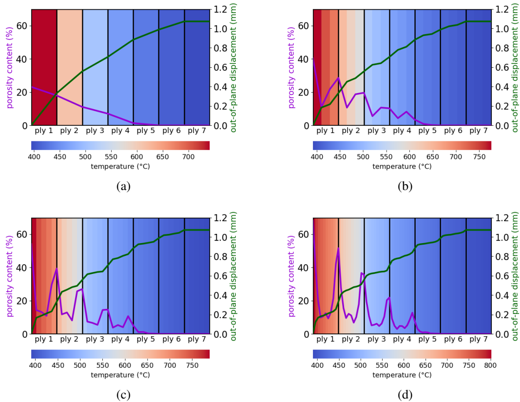
Figure 4.19. – Evolution of the numerically modelled out-of-plane displacement and porosity content in each plies after exposure to a 116\text{kw/m}^2 heat flux for 60s. Each ply discretized into a different amount of subvolumes: (a) 1, (b) 3, (c) 5 and (d) 10
