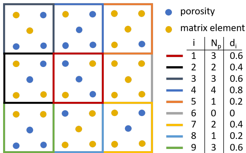
Figure 3.22. – 2D illustration of the porosity distribution within the boxes of a 2 nd order local domain considering a box size of 5 elements. Calculation of the porosity density of the boxes forming the local domain
