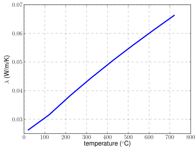
Figure 4.17. – Evolution of the porosity thermal conductivity with temperature
