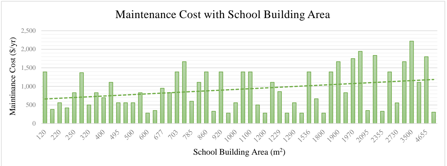
Figure 5.13. The maintenance cost of selected schools with the school building area.
