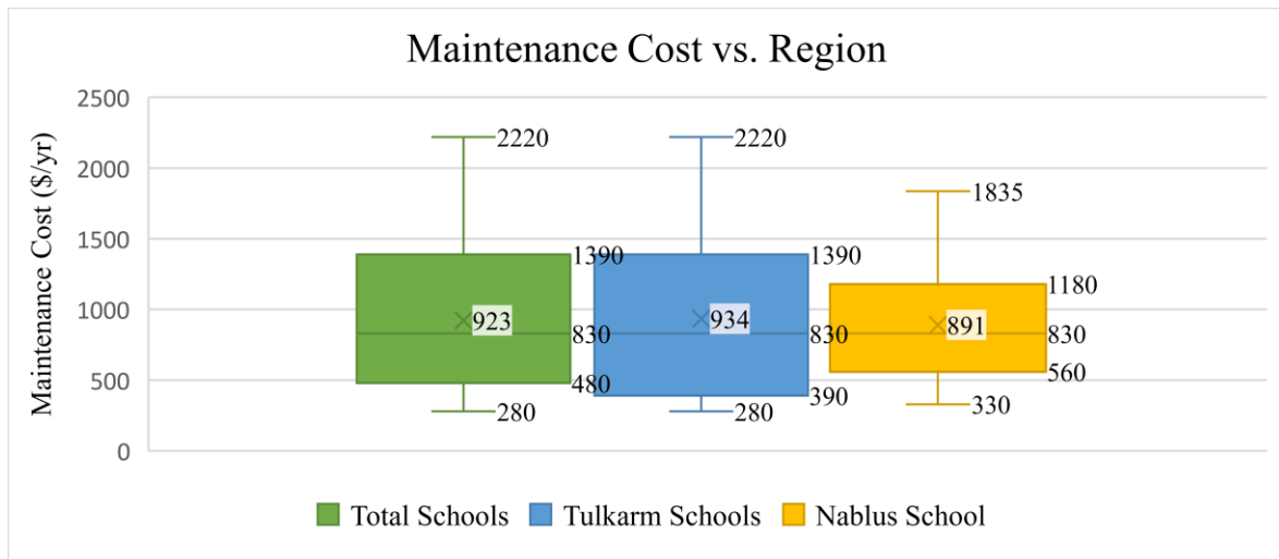
Figure 5.16. The maintenance cost in all schools compared with Tulkarm and Nablus schools.
