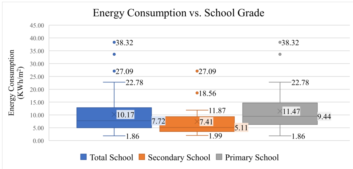
Figure 5.3. The energy consumption in all schools comparing with secondary and primary schools.
