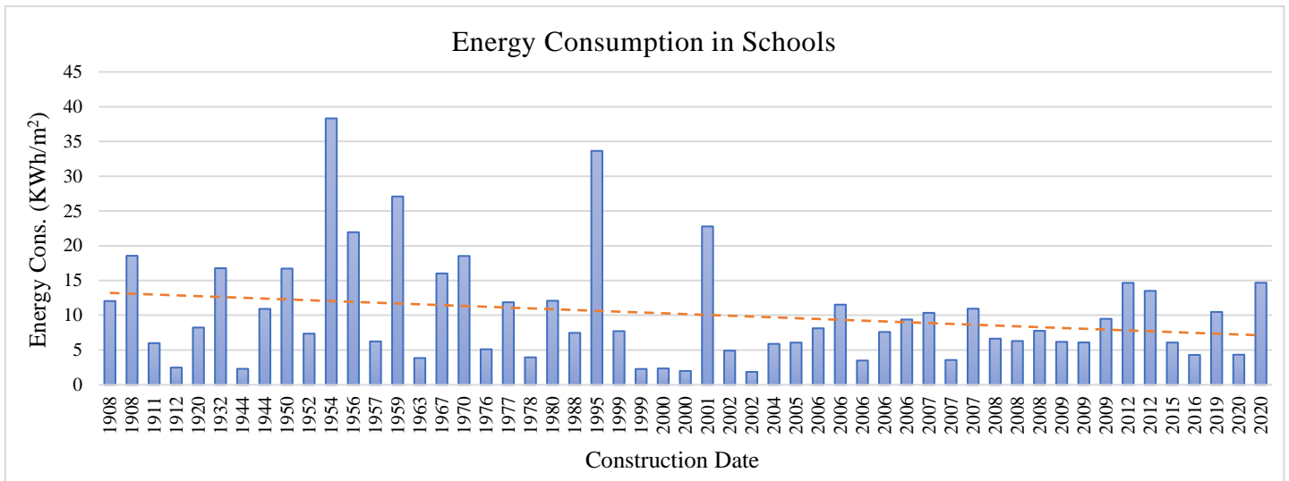
Figure 5.1. Energy consumption in schools with the construction date.
