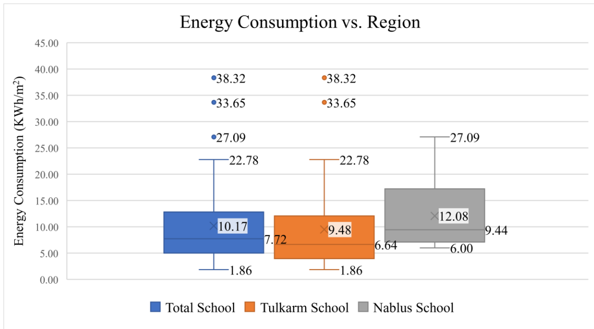
Figure 5.5. The energy consumption in all schools comparing with Tulkarm and Nablus schools.
