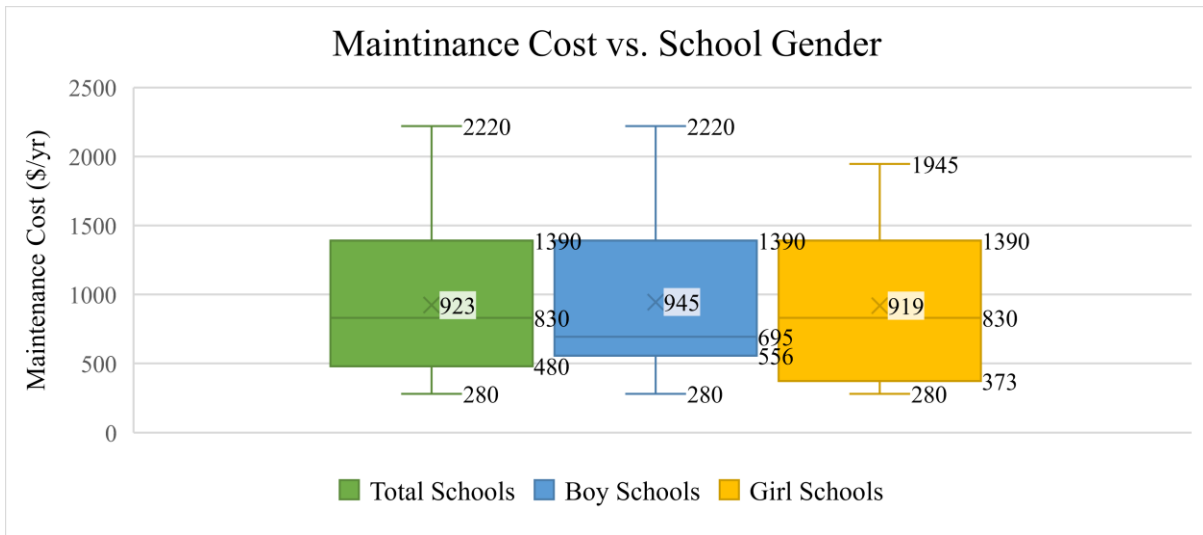
Figure 5.14. The maintenance cost in all schools comparing with boy and girl schools.
