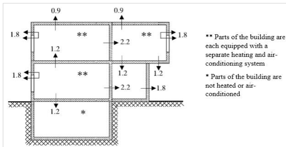
Figure 3.2. The required thermal transmittance ( W/m^2.K ) for walls and floors in the building. Source: (Palestinian Energy Code, 2004)
