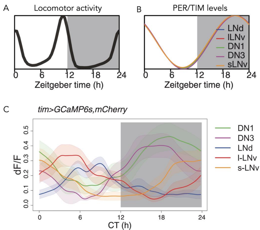
Figure 1.13 Non-synchronous intracellular Ca^{2+} rhythms exhibited by Drosophila pacemaker neurons in vivo. A: Schematic representation of bimodal activity pattern displayed by Drosophila melanogaster in 12:12 LD conditions. The multi-oscillator network of the Drosophila brain clock drives activity around dawn (M peak) and dusk (E peak). B: Schematic representation of the expression levels of PER and TIM proteins in different clock neuron clusters. C: Average fluorescence displayed by the Ca^{2+} sensor GCaMP6s expressed in cell bodies of five clock groups (color-coded) over a period of ~24
