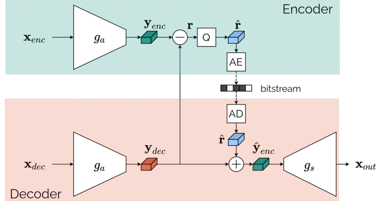
Figure 5.7: Latent-domain residual.
