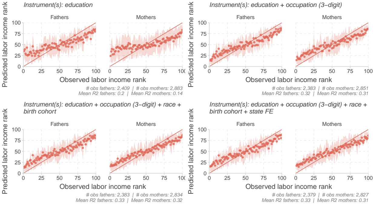
Figure B.9. Observed vs. (out-of-sample) predicted individual labor income rank
