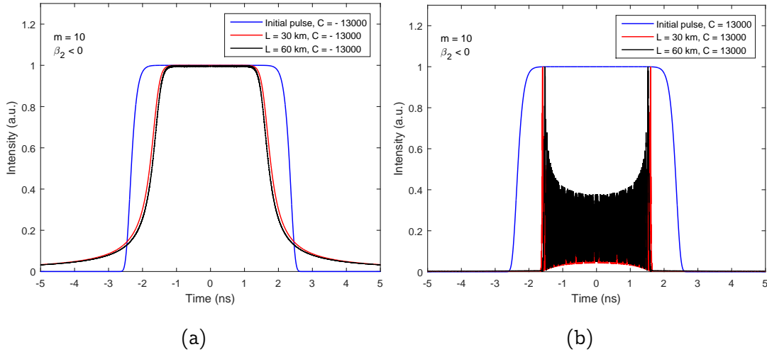
Figure A.13: (a) Temporal trace of the initial rectangular pulse, with a negative initial chirp parameter C = -13000 , in blue, and after propagating through 30 km and 60 km of SMF28 in red and black, respectively. (b) Same temporal traces for a positive C = +13000 .
