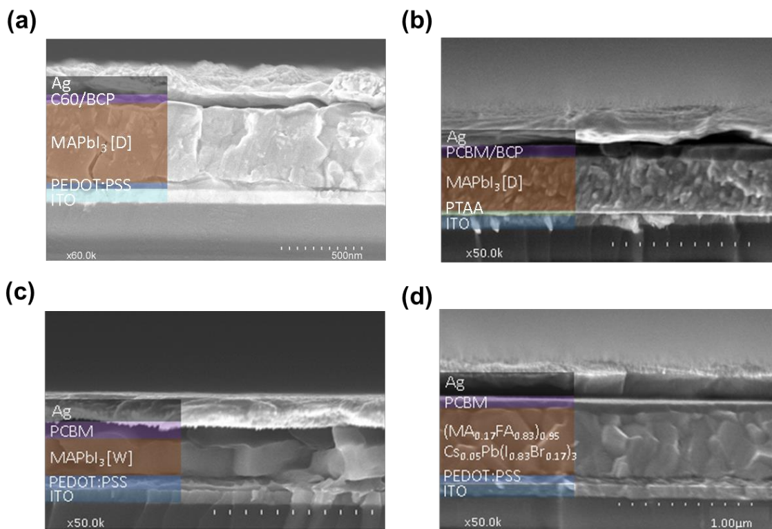
Figure 4.7 Cross-section SEM images of the structures (a) dry MAPbI 3 with PEDOT:PSS (i), (b) dry MAPbI 3 with PTAA (ii), (c) wet MAPbI 3 (iii) and (d) 3CP (iv), respectively.
