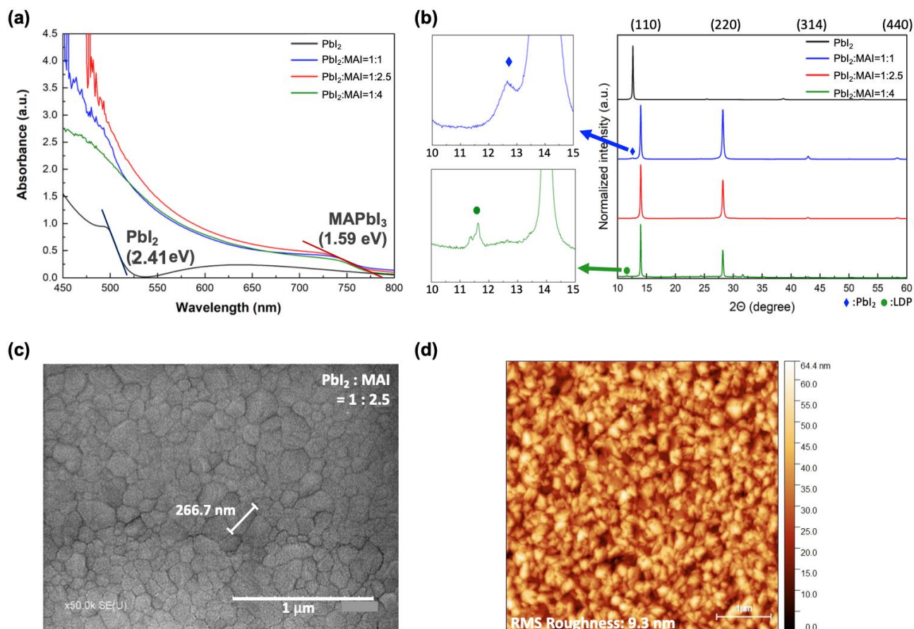
Figure 3.8 (a) Absorbance graph and (b) XRD patterns of PbI 2 and perovskite thin films deposited by co-evaporation with the deposition ratio of 1:1, 1:2.5, and 1:4. (c) SEM and (d) AFM image of MAPbI 3 film prepared with optimized condition (1:2.5).
