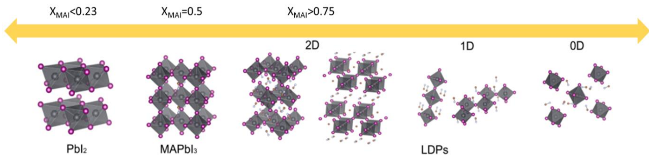
Figure 3.9 Crystal structures of PbI 2 and MAPbI 3 perovskites in the form of 3D perovskite, 2D, 1D and 0D LDP where X_{MAI} defines the mole fraction of MAI in the mixture of MAI and PbI 2 ( X_{MAI} = n_{MAI} / (n_{MAI} + n_{PbI2}) ) [173].
