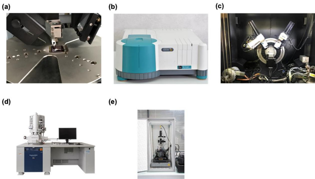
Figure 3.6 Photographs of (a) profilometer, (b) UV-Visible spectrophotometer (Cary 50), (c) XRD (D8 Discover), (d) scanning emission microscope MEB HITACHI, (e) AFM (PicoScan 3000).
