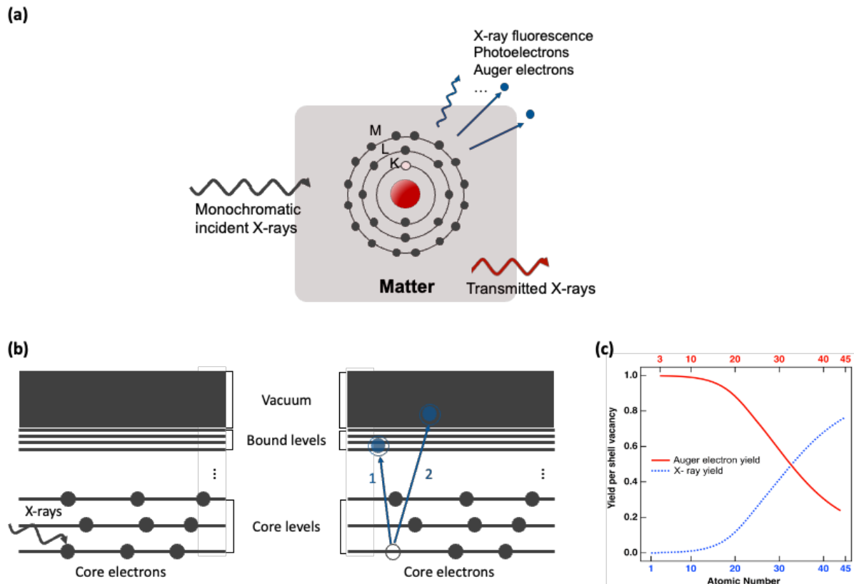
Figure 2.20 Schematic of (a) interaction between X-rays and matter and (b) absorption process where processes 1 and 2 indicate the transfer of a photoelectron into a bound level and vacuum level, respectively. (c) Graph of Auger electron and fluorescence yield with respect to atomic number Z for the K shell. Courtesy of http://www.wikiwand.com/en/Auger_electron_spectroscopy .
