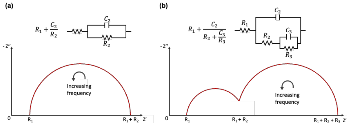
Figure 4.4 Equivalent circuit model of (a) R_1 + C_2/R_2 and (b) \{R_1 + C_2/(R_2 + C_3/R_3)\} .
