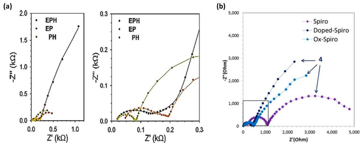
Figure 1.10 (a) Full and zoomed Nyquist plot of PSCs (FTO/ \text{TiO}_2 /perovskite/spiro-OMeTAD/Au), electron-only device with \text{TiO}_2 , and hole-only device with spiro-OMeTAD [63]. (b) Complex impedance plot of undoped, doped and oxidized spiro-OMeTAD based PSCs [64].
