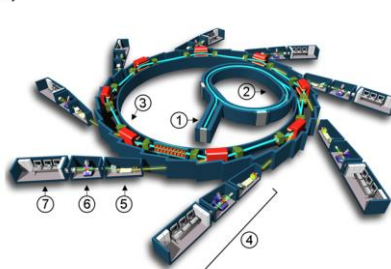
Figure 2.17 (a) A view of the synchrotron facility, SOLEIL in France. (b) Structure of third-generation 2.75 GeV Soleil Light Source at Saint-Aubin, France. It consists of (1) the injector, (2) the booster ring, (3) the storage ring, (4) an experimental station called “beamline”, including (5) optics hutch, (6) experimental hutch, and (7) control room.
