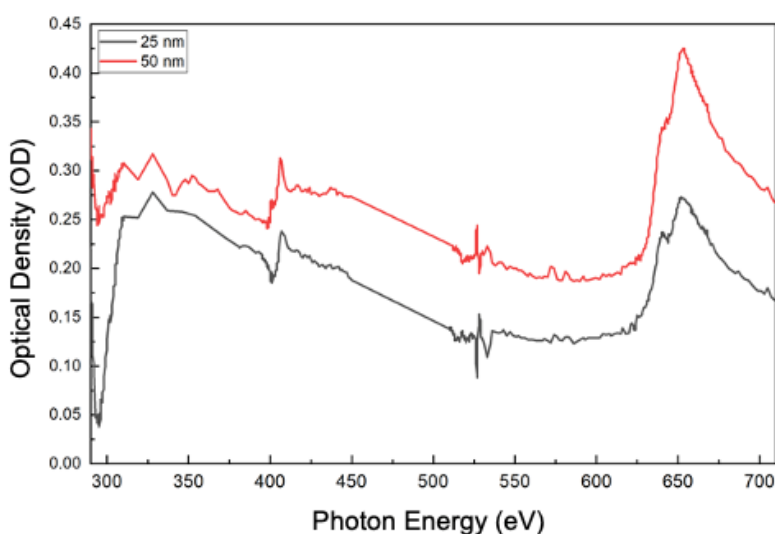
Figure 5.10 Experimental NEXAFS spectra of MAPbI 3 with different thicknesses.
