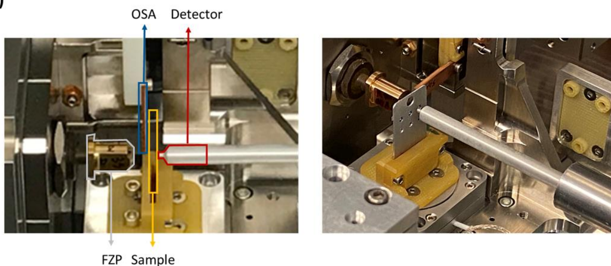
Figure 5.3 Scheme of the STXM technique. (b) Close-up interior view of the STXM instrument.
