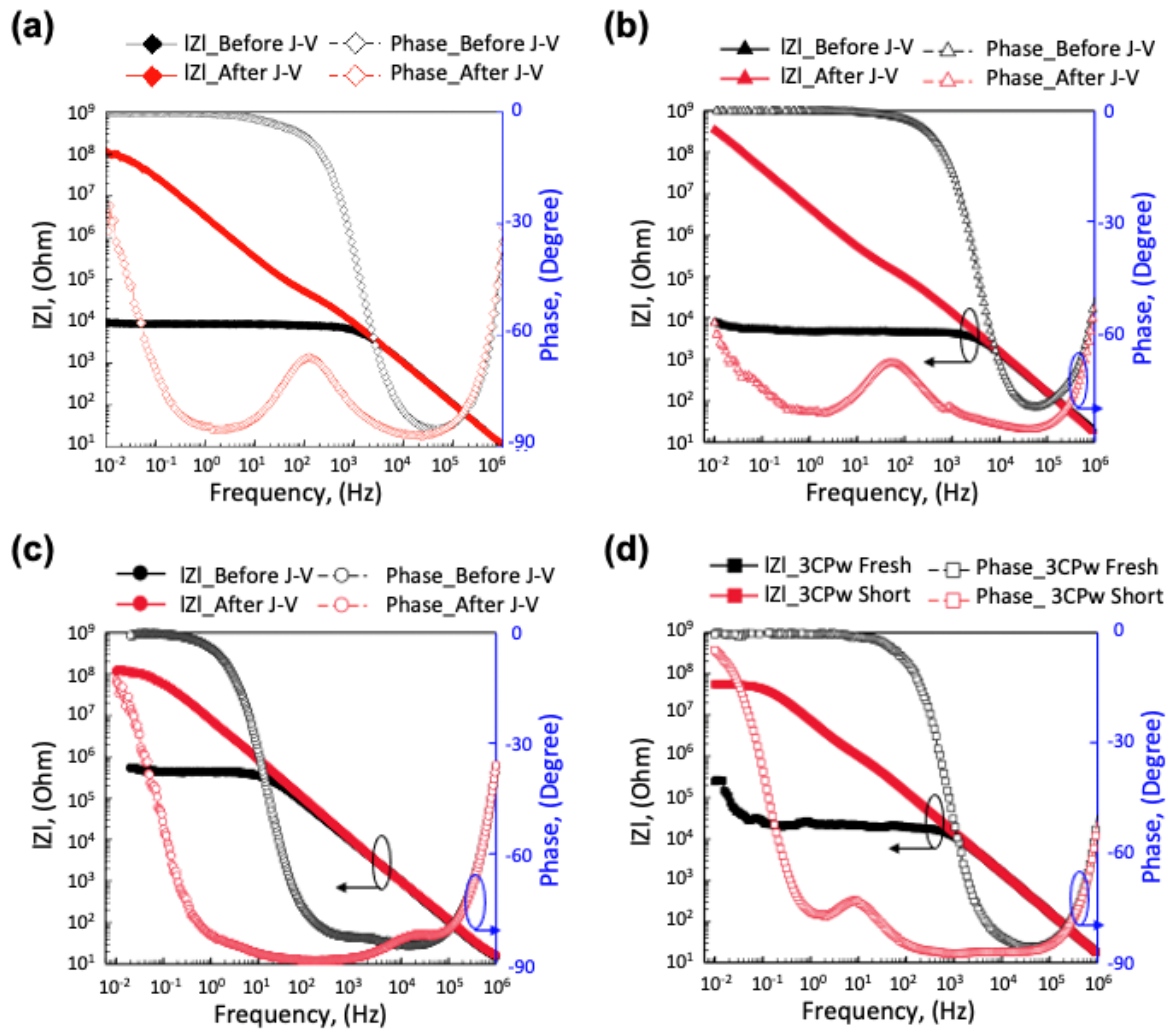
Figure 4.11 Bode impedance and phase plot of the different devices before and after applied electric field under dark conditions; co-evaporated MAPbI 3 on (a) PEDOT:PSS (i) and (b) PTAA (ii), (c) spin-coated MAPbI 3 (iii) and (d) 3CP (iv) (Short means shorting conditions.).
