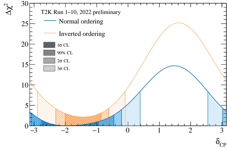
Figure 7.16: One-dimensional negative log-likelihood in \delta_{\text{CP}} for normal (blue) and inverted (orange) ordering using reactor constraints of Reference [12], and the shaded regions correspond to confidence levels obtained with the Feldman – Cousins method.
