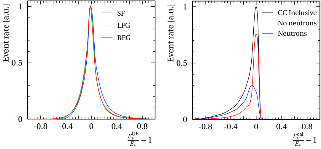
Figure 3.13: Left: resolution and bias of the neutrino energy estimator E_{\nu}^{\text{QE}} for CCQE events when using RFG, LFG and SF models. Right: resolution and bias of E_{\nu}^{\text{cal}} for all CC events with the contributions from events with (blue) and without (red) neutrons in the final state using the MINERvA flux (shown in Figure 3.1) with the NEUT event generator.
