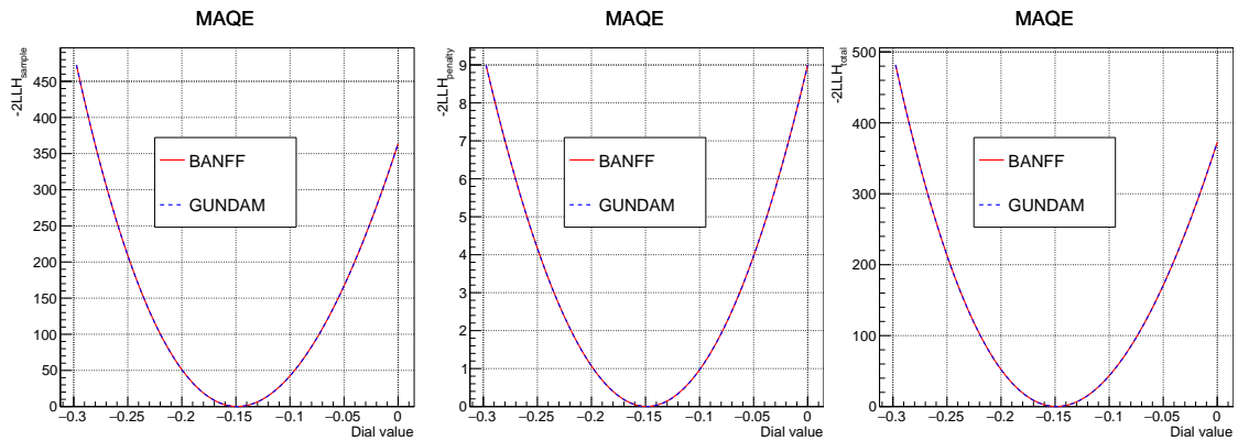
Figure 8.2: One example of the 712 likelihood scan comparisons of the statistical part -2 \log \mathcal{L}_{\text{stat}} (left) and the penalty term -2 \log \mathcal{L}_{\text{sys}} (center) separately, as well as the total likelihood -2 \log \mathcal{L}_{\text{tot}} (right) for the M_A^{\text{QE}} parameter.
