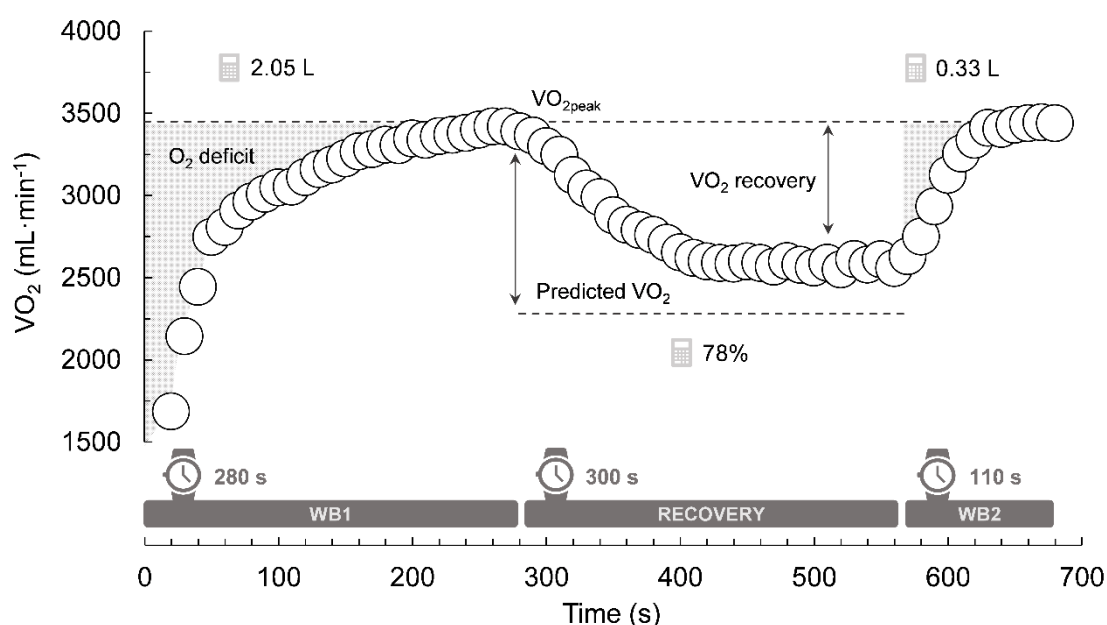
Figure 1 Representative example showing the \dot{V}O_2 response of a participant who performed the 5-min recovery condition. The figure illustrates the calculation of the O 2 deficit of WB1 and WB2, and the quantification of the \dot{V}O_2 recovery between both work bouts.
