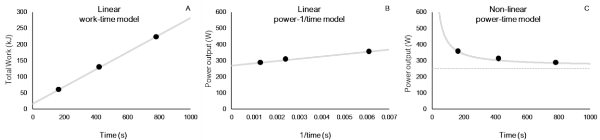
Figure 5 Regression analyses and curve fits for each of the three two-parameter mathematical models that are commonly used to determine CP and W' : (A) linear work-time model, (B) linear power- 1/\text{time} model and (C) non-linear or hyperbolic power-time model.
