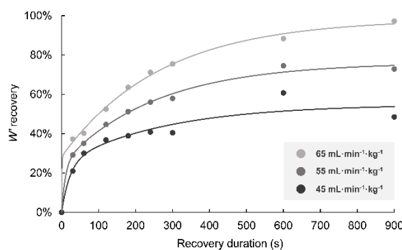
Figure 6 Model-predicted W' recovery for a hypothetical athlete with either a low ( 45 \text{ mL} \cdot \text{min}^{-1} \cdot \text{kg}^{-1} ), medium ( 55 \text{ mL} \cdot \text{min}^{-1} \cdot \text{kg}^{-1} ) or high ( 65 \text{ mL} \cdot \text{min}^{-1} \cdot \text{kg}^{-1} ) \dot{V}O_{2peak} .
