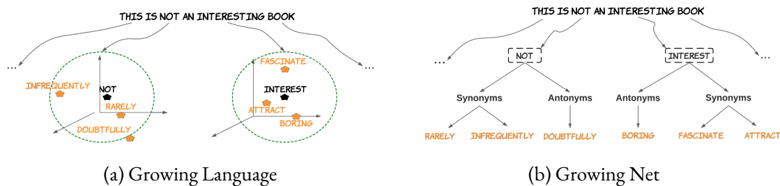
Figure 3.4 – The mechanism employed to generate sets of potential word replacements in Growing Language involves embedding words from the target text into a latent space and capturing nearby words in this space. Conversely, Growing Net leverages the tree structure of WordNet to create sets of potential word replacements.
