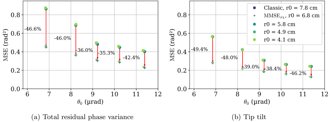
Figure 4.20: Absolute value of the MSE for the classical case (circles) and the \text{MMSE}_{\phi_\chi} case (crosses) versus \theta_0 , for different r_0 . Each color depicts a different r_0 . Red arrows correspond to the MSE reduction provided by the \text{MMSE}_{\phi_\chi} method, with the reduction value on its left. (a) Total MSE error over the AO corrected modes. (b) MSE error on tip and tilt.
