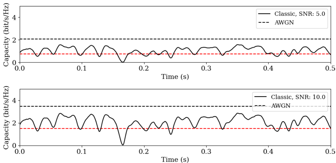
Figure 7.4: Capacity time-series of the uplink pre-compensated channel, with classical pre-compensation, in the MOSPAR 9090 case. The AWGN capacity is represented in black dashes, and the rate threshold in red dashes.
