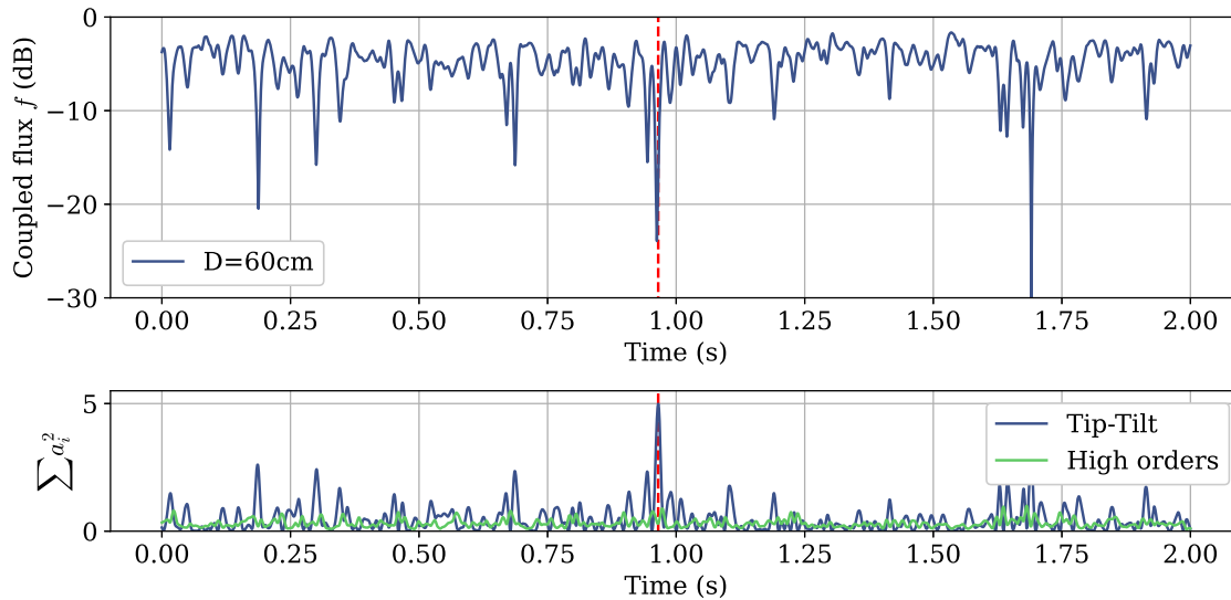
Figure 3.32: Time-series in the 60 cm aperture case (at the top) compared with the instantaneous sum of the square Zernike projections (at the bottom), separated in the sum of the low orders and high orders, in the MOSPAR 9090 turbulence case.
