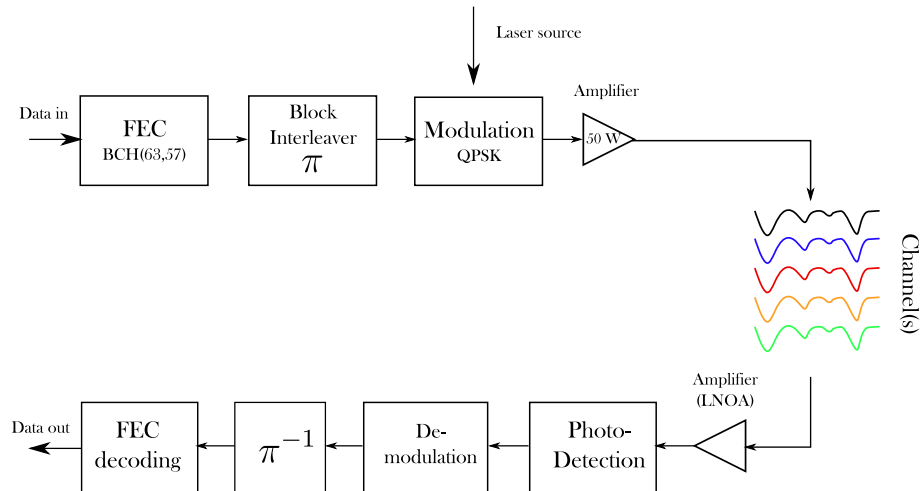
Figure 7.18: Considered E2E transmission chain in the numerical assessment of the BER for the AO ground to satellite pre-compensated channel.
