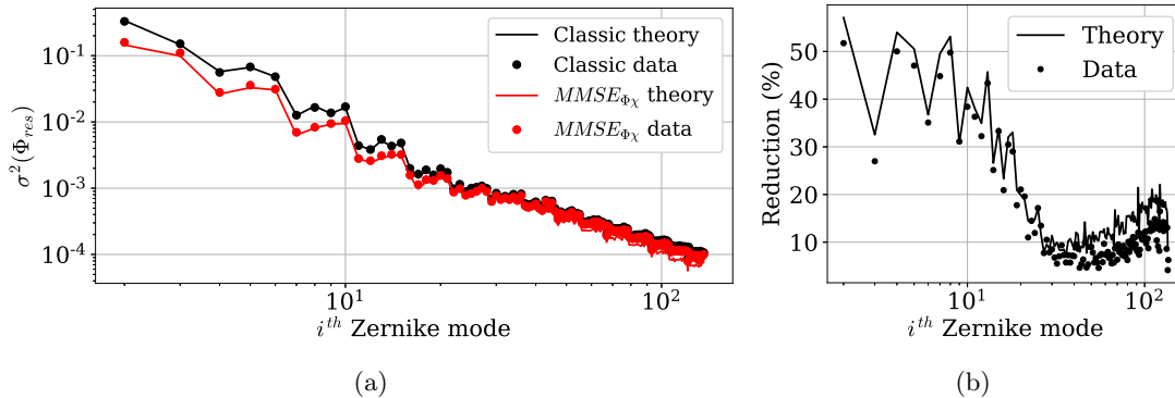
Figure 4.10: On the left, modal residual phase variance function of the mode number for the classical pre-compensation and the MMSE_{\Phi\chi} estimation method, computed theoretically and from data for the MOSPAR 9090 turbulence case. On the right, modal reduction function of the mode.
