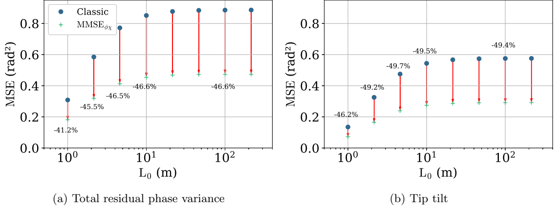
Figure 4.18: Red arrows correspond to the MSE reduction provided by the MMSE _{\phi\chi} method, with the reduction rate below the arrow. (a) Total MSE error over the AO corrected modes, (b) MSE error on tip and tilt.
