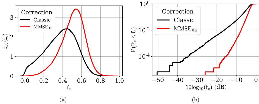
Figure 4.13: Coupled flux statistics for MOSPAR 9090 at 30° elevation, D=60 cm and L_0=20 m. The two correction cases are depicted: classic in black, \text{MMSE}_{\Phi_\chi} in red.
