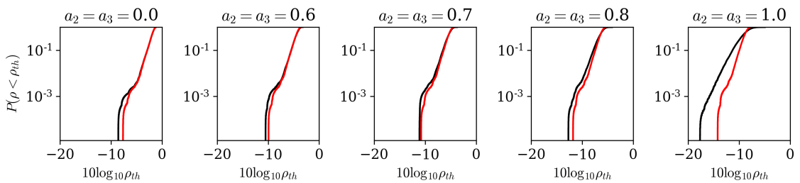
Figure 7.28: Comparison of the exact and approximated coupled flux. The black curve depicts the exact coupling, and the red curve the coupling approximation. It is computed for a fixed tip and tilt value, and varying high order modes, in the MOSPAR 9090 turbulence case.
