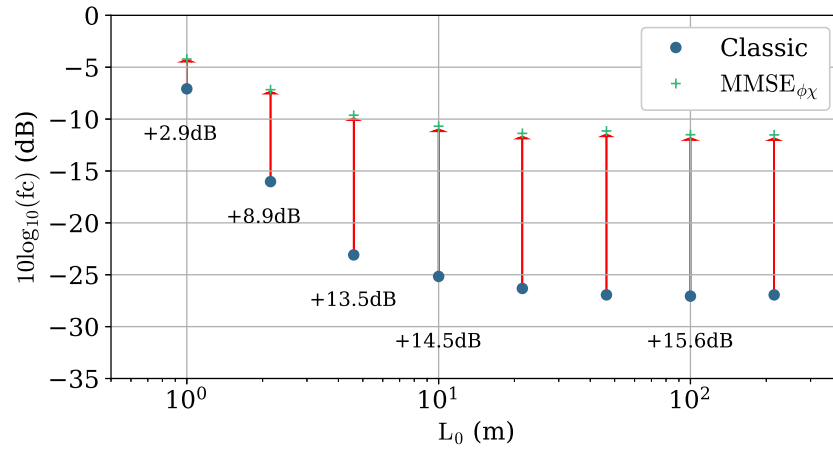
Figure 4.19: Absolute value of the CDF at P(f_c \leq F_c) = 10^{-3} for the classical case (blue circles) and the MMSE _{\phi\chi} case (green crosses) versus L_0 . Red arrows correspond to the gain at probability 10^{-3} on the CDF provided by the MMSE _{\phi\chi} method, with the gain value given below the arrow.
