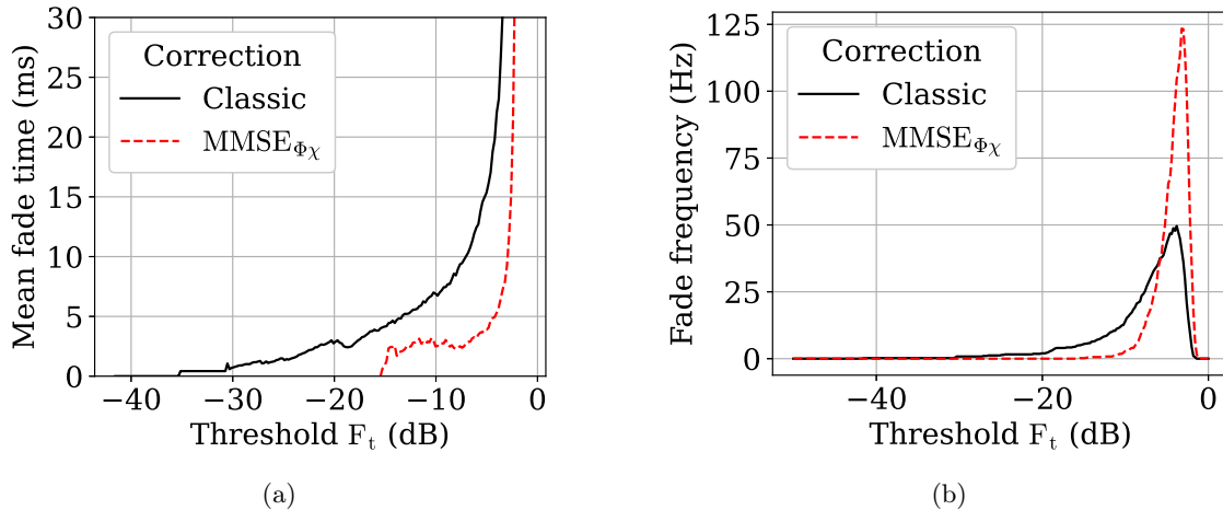
Figure 4.16: Mean fade duration (a) and fade frequency (b) function of the coupled flux threshold F_t for the classical pre-compensation case and the MMSE_{\Phi_X} estimated case in the MOSPAR 9090 turbulence case.
