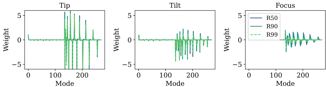
Figure 4.28: Three first rows of the estimator computed for the profiles MOSPAR 5050, 9090 and 9999.
