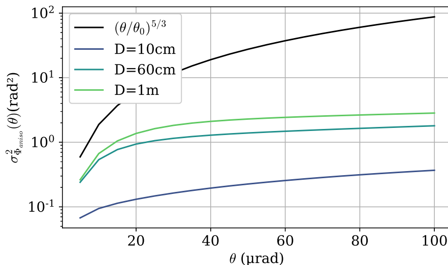
Figure 2.17: Comparison between the phase variance by Fried and the phase variance by Chassat, function of the angular separation \theta , for the following integrated parameters: \theta_0 = 6.83 \mu\text{rad} , r_0 = 4.1 \text{ cm} , \sigma_\chi^2 = 0.08 .
