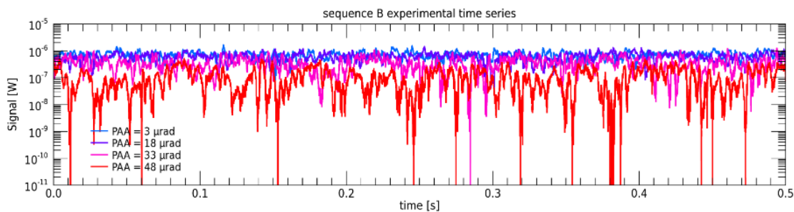
Figure 2.20: Illustration of time-series of the pre-compensated FEEDELIO uplink, function of the angular decorrelation[89]
