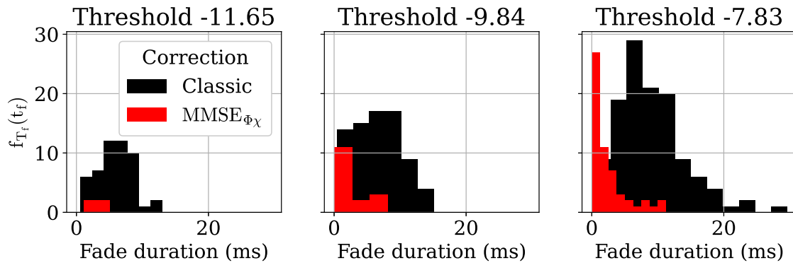
Figure 4.17: Fade duration distribution for 3 different arbitrary thresholds for the classical pre-compensation case and the MMSE_{\Phi_X} estimated case in the MOSPAR 9090 turbulence case.
