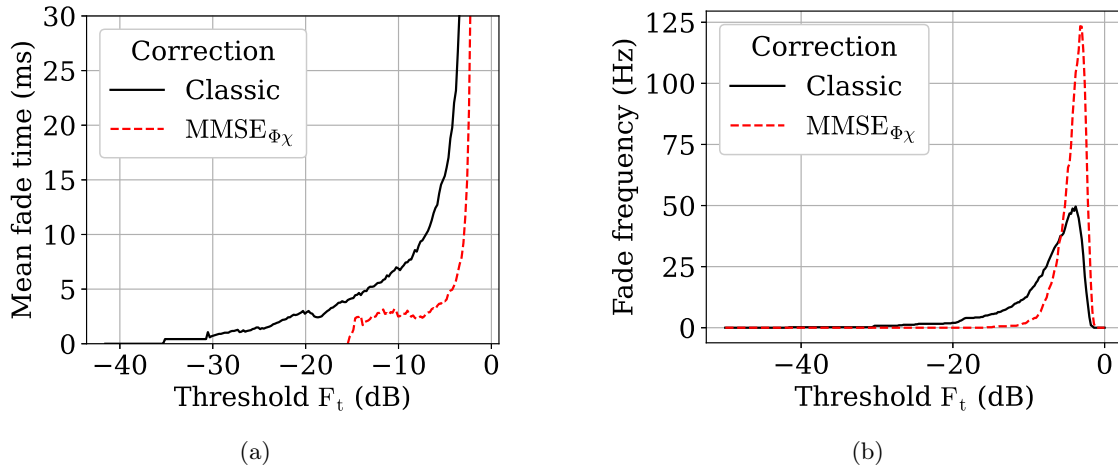
Figure 4.16: Mean fade duration (a) and fade frequency (b) function of the coupled flux threshold F_t for the classical pre-compensation case and the MMSE_{\Phi\chi} estimated case in the MOSPAR 9090 turbulence case.
