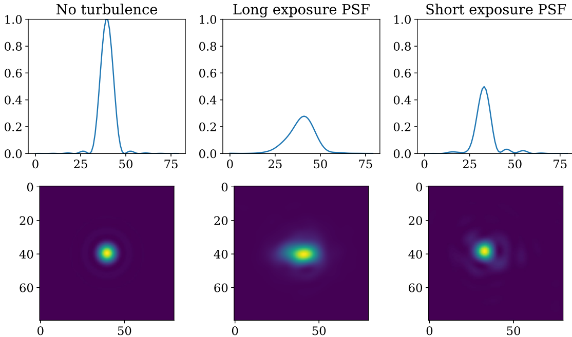
Figure 2.19: Anisoplanatic PSF compared to an Airy pattern. On the left: Airy pattern (PSF with perfect plane phase), center: Long exposure anisoplanatic PSF (averaged on 0.1 s), right: short exposure anisoplanatic PSF. Top: centered slice, bottom: image in the focal plane.
