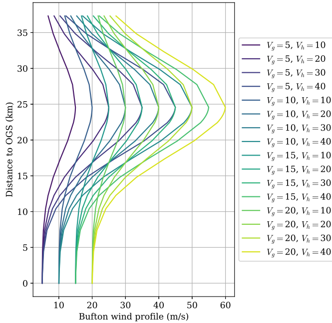
Figure 5.18: Bufton wind speed profile (m/s) function of the distance to the OGS on the line of sight, for different combinations of ground layer and tropopause wind speed.
