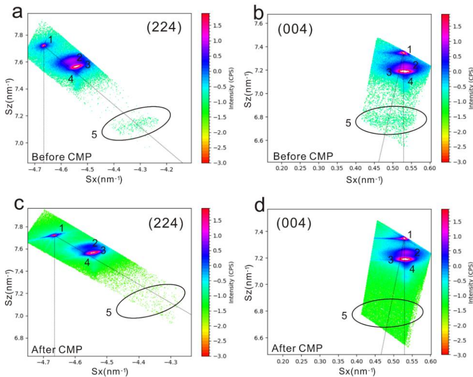
Figure 3.9 X-Ray diffraction reciprocal space mappings around (224) and (004) reflection on the sample before and after CMP. The black dotted vertical and inclined lines represent respectively the full strain lines and full relaxation lines.
