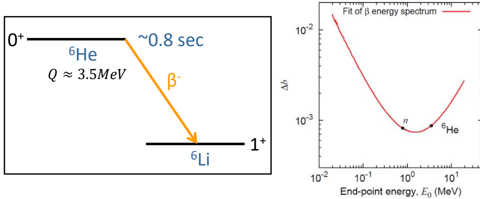
Figure 1.6: Left panel: the decay scheme of the {}^6\text{He} \beta -decay. Right panel: the 1\sigma statistical uncertainties of the Fierz interference term obtained by fitting the simulated \beta -energy spectra with different values of the endpoint energy. Figure taken from Ref. [46].
