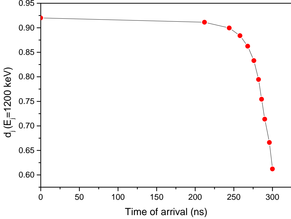
Figure 3.22: The probability of a pileup event to be above the energy threshold (1200 keV in this example) against the time of arrival of the second signal relative to the first one.
