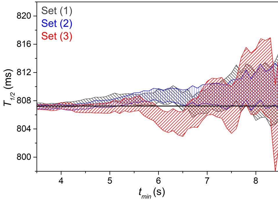
Figure 3.30: Half-life estimate obtained for Set1, Set2 and Set3 of measurements (respectively in grey, blue and red) as a function of the lower bound of the fitting range T_{min}^{Fit} . The colored areas indicate the values covered by the statistical error bars given at one standard deviation.
