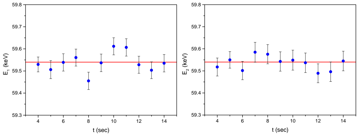
Figure 3.10: Centroids of the 59.54 keV photopeak against time within the decay cycles after calibration with gain and baseline corrections for Det1 (left panel) and Det2 (right panel) for one run of Set1. The red line represents 59.54 keV
