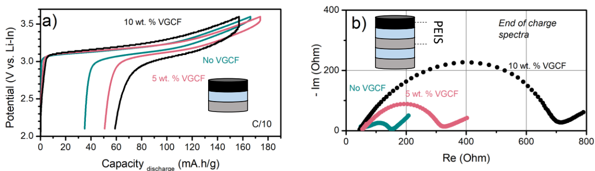
Figure 2.2: (a) First cycle at C/10 using NMC 622 + \text{Li}_6\text{PS}_5\text{Cl} (70/30 wt. % ratio) as cathode composites with 5 wt. % or 10 wt. % additional VGCF, or without VGCF. A loading of 16 \text{ mg/cm}^2 of composite is used. (b) Composites of same formulation are implemented in three electrode setup, to take PEIS measurements at the end of the first charge (3.6 V vs. Li-In/In) at C/10, 10 hours of relaxation is made prior the measurements.
