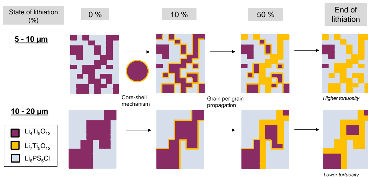
Figure 3.16: Proposed schematic of lithiation pathway in LTO composites
