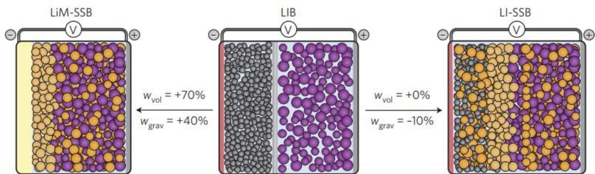
Figure 1.2: Typical battery architectures for the conventional lithium-ion and solid-state batteries. The volumetric and gravimetric energy densities are represented by w_{\text{vol}} and w_{\text{grav}} , respectively. Reproduced from reference 26 .
