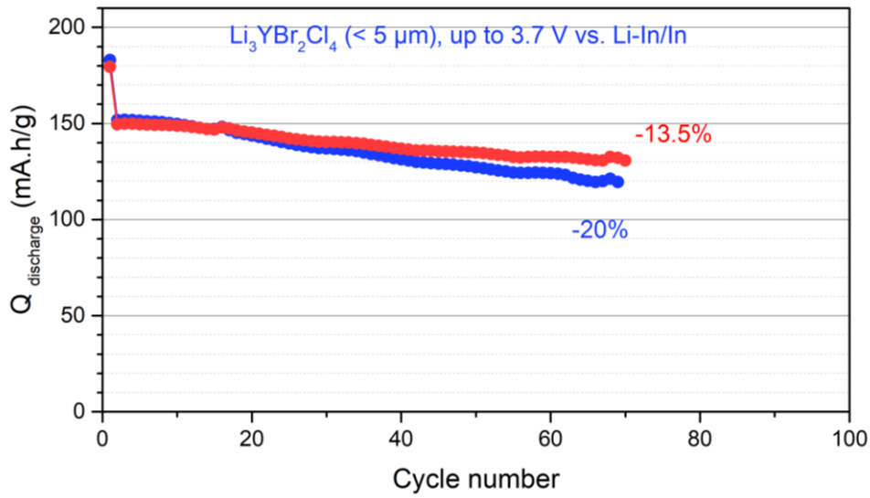
Figure S4.16: Capacity retention up to 3.7 V vs. Li-In/In of two NMC 811 (MSE) + LYBC (< 5 μm) in a 70/30 wt. % ratio with an additional 1.5 wt. % VGCF. First cycle is made at C/10 and is followed by C/2 cycling.
