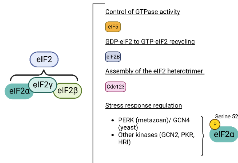
Figure 16: eIF2 known partners. As a key component of translation initiation, eIF2 activity is regulated by a number of partners that control its GTPase activity (eIF5), its recycling from a GDP inactive form to a GTP-bound active form (eIF2B), its assembly (Cdc123), and partners that modify specific residues (S52 in subunit \alpha ) upon specific stress-related responses.
