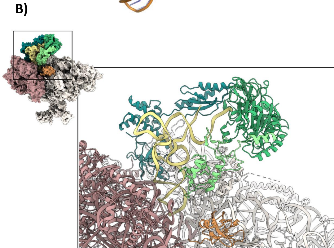
Figure 15: A) Structure of the S. solfataricus ternary complex. Domain III of aIF2 \alpha is shown in blue, domain I of aIF2 \beta is shown in pink, and aIF2 \gamma is shown in different shades of green. PDB:3V11. B) Structure of eIF2 on the 43S PIC.
