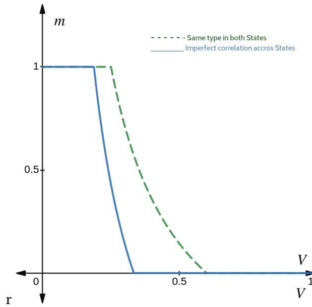
Fig. 3.11. Type correlation and optimal strategies
