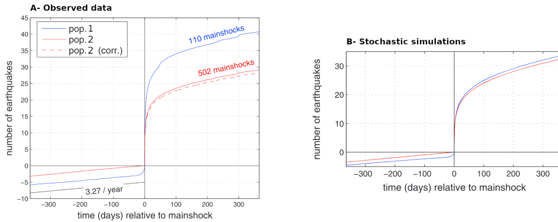
FIGURE 1.16: A. Stacked and averaged number of M \geq 4 earthquakes within 50 km of the mainshock epicenter, for the two populations 1 (accelerated foreshock seismicity) and 2 (non-accelerated). Red dashed line: aftershocks of population 2 after correcting for a difference in magnitude distribution for the two populations. B- Same as A. but with synthetic ETAS earthquake catalogs, modeling a cascading earthquake triggering process. Modified from Marsan et al. (2014)
