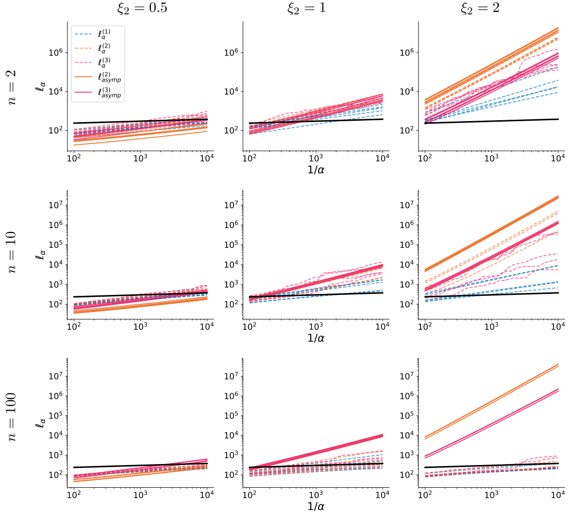
Figure 4.1: On each plot, five replications of return level estimators \hat{\ell}_\alpha^{(i)} for i \in \{1, 2, 3\} (dotted lines), and the asymptotic expressions of \hat{\ell}_\alpha^{(2)} and \hat{\ell}_\alpha^{(3)} (plain lines), for a dataset with n observations following a GPD with (\sigma_0, \xi_0) = (15, 0.1) (the black lines represent the real return level). Each row represents a choice of n \in \{2, 10, 100\} , and each column a choice of the support upper bound of the prior on \xi : \xi_2 \in \{0.5, 1, 2\} .
