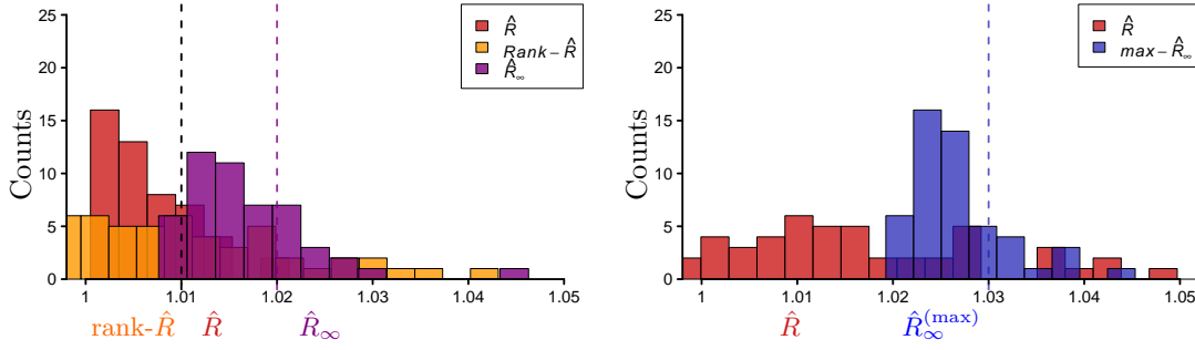
Figure 3.9: Behaviour of multivariate and univariate \hat{R}_{\infty} on the Bayesian logistic regression example, with m = 4 chains of size n = 200 . On the left: Histograms of 50 replications of \hat{R} , rank- \hat{R} and univariate \hat{R}_{\infty} all applied on the log-posterior. On the right: Histograms of 50 replications of Brooks–Gelman \hat{R} and \hat{R}_{\infty}^{(\max)} . The dashed line corresponds to different thresholds: on the left, 1.01 in black for \hat{R} and rank- \hat{R} , 1.02 in violet for \hat{R}_{\infty} , and on the right 1.03 in blue for \hat{R}_{\infty}^{(\max)} .
