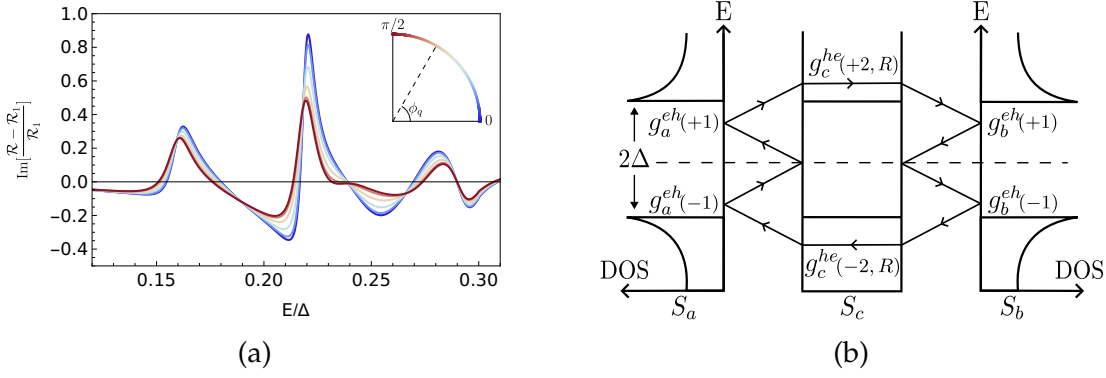
Figure 4.17: (a) Variation of the spectral function \text{Im}\left[\frac{\mathcal{R}-\mathcal{R}^{(1)}}{\mathcal{R}^{(1)}}\right] . Different colors represent a different quartet phase, \phi_q \in [0, \frac{\pi}{2}] , as explained in the inset. Other parameters are set to \omega_0 = 0.7 \Delta , \Gamma_j = 0.5 \Delta , R = 25 \xi_0 . (b) Sketch of an octet process \Sigma_0^{-,e_1 h_2} \times \Sigma_0^{+,e_2 h_1} , which couples a hole at energy E_0 on dot 1 to an electron at the same energy on dot 2 and accumulates a phase e^{2i\phi_q} .
