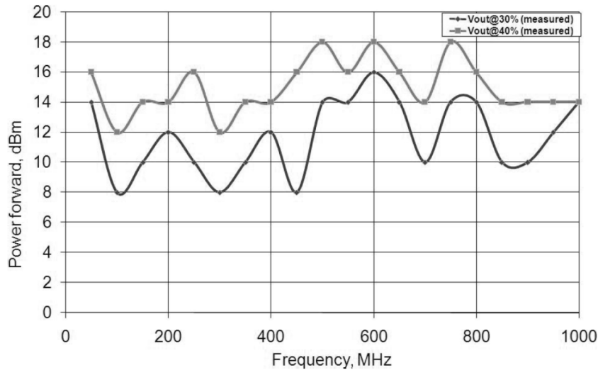
FIGURE 1.6 – DPI test result for evaluating the conducted immunity level of an IC under test at different failure criterion [17].
