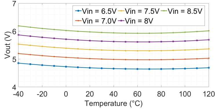
FIGURE 2.2 – Output voltage as a function of temperature and input voltage variation.
