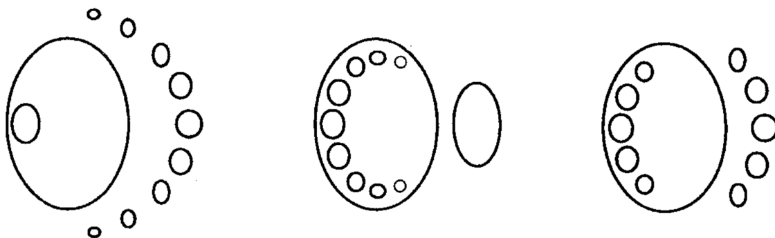
Figure 1.1: Maximal projective curves of degree 6.
