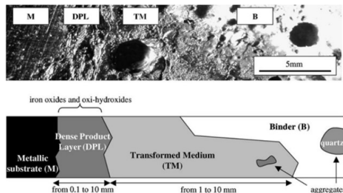
Figure I-25. Photography and schematic representation of the two corrosion products layers, surrounded by the rebar steel and the binder [176].
