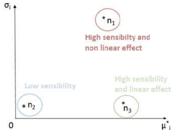
Figure 0-13 Results example of a sensitivity analysis realised with the Morris method [6].
