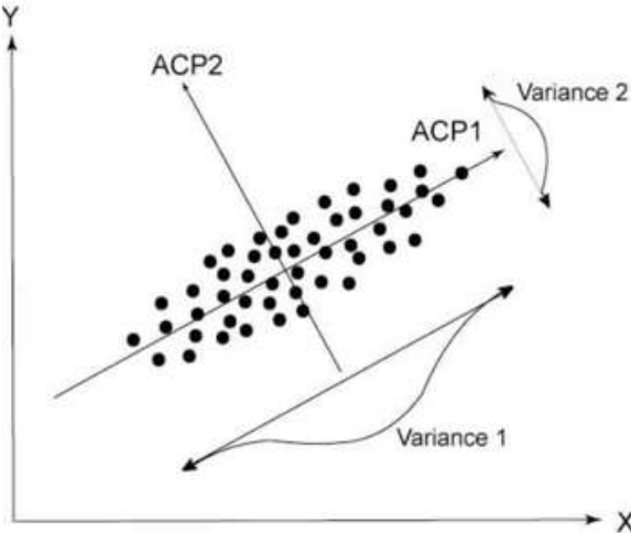
Figure 0-12 Example of graphical representation for principal component analysis exploitation [445].
