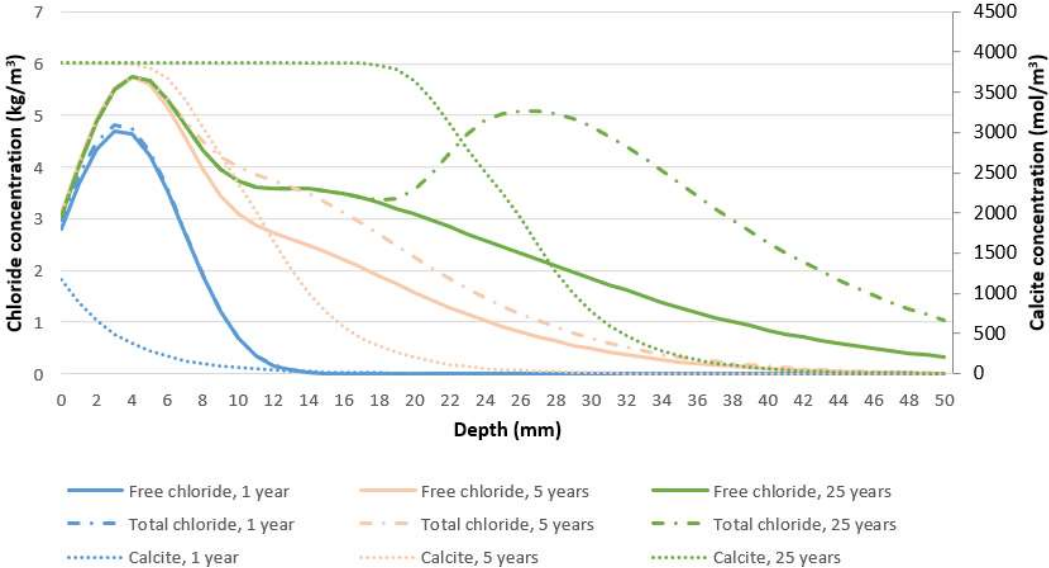
Figure III-27 Free and total chloride concentrations (kg/m 3 ) compared to the calcite concentrations (mol/m 3 ) in the material after 1, 5 or 25 years.
