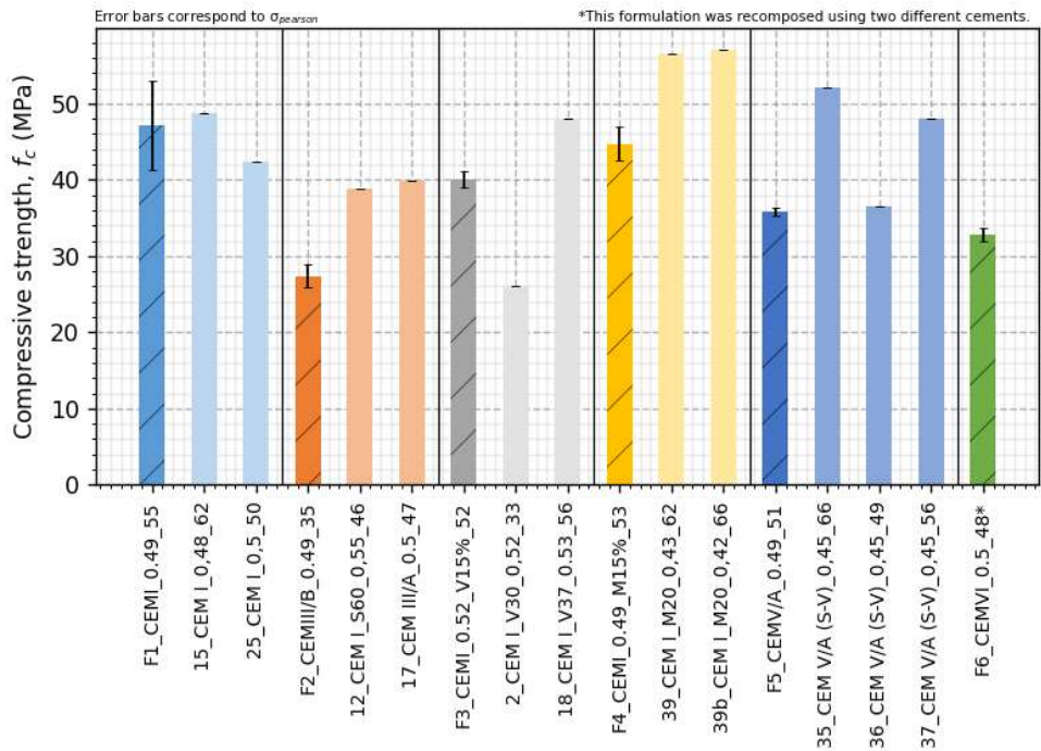
Figure II-6 Compressive strength values obtained after 28 days in dry conservation for the PhD mixes and the closest formulations presented in the National project PerfDuB.
