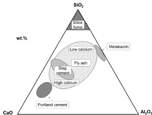
Figure I-3 Ternary diagram of Portland cement and supplementary cementing materials [48].
