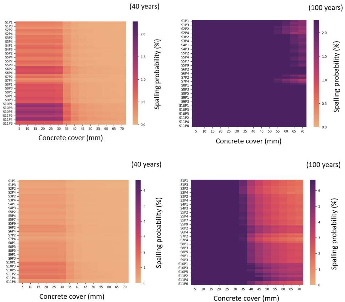
Figure IV-46 Corrosion-induced spalling probability obtained after 40 and 100 years of exposure, considering a threshold of 2.27% ( \beta=2 ) and 6.68% ( \beta=1.5 ).
