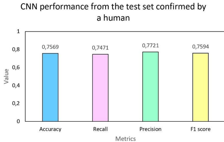
Figure 4. CNN performance metrics based on a test set consisting of a total of 800 images, which were validated by a human expert.
