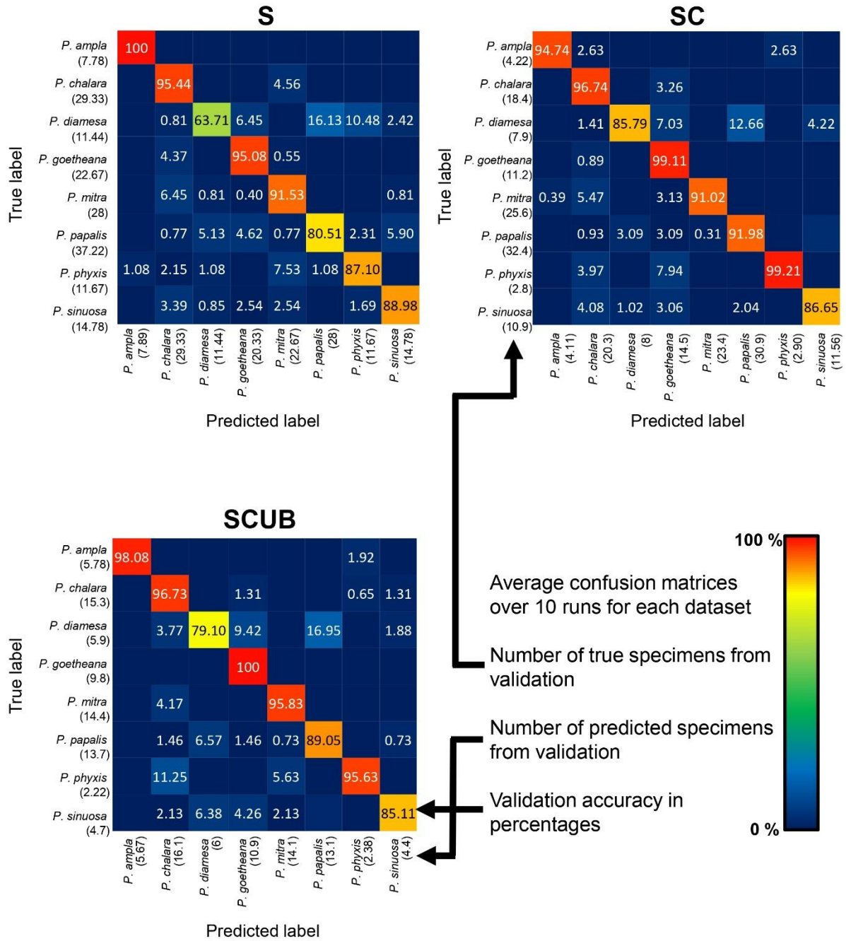
Figure 5. Average confusion matrices for the “S”, “SC” and “SCUB” dataset. The numbers inside the matrices shows the average validation accuracy of specimens in each class that has been correctly or incorrectly classified. The numbers under each species name are the total number of true or predicted labels.
