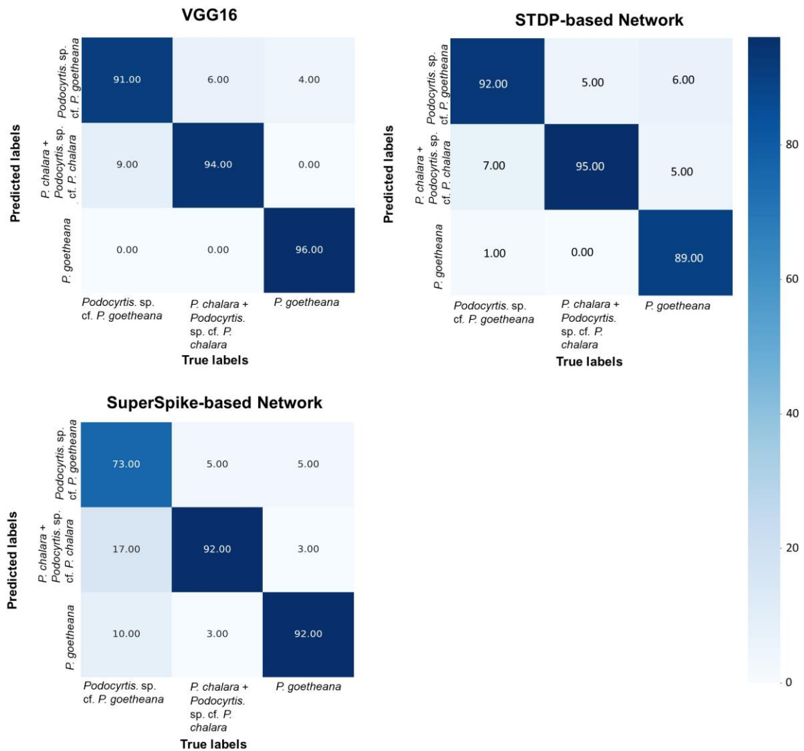
Figure 4. Examples of confusion matrices obtained from random single runs – Analyses of 3_classes dataset with VGG16, STDP-based SNN and SuperSpike-based SNN. Correct assignments were reached in 92.60 %, 90.40 % and 84.42 % of the cases in VGG16, STDP-based SNN and SuperSpike-based SNN, respectively. The color scale indicates the number of specimens.
