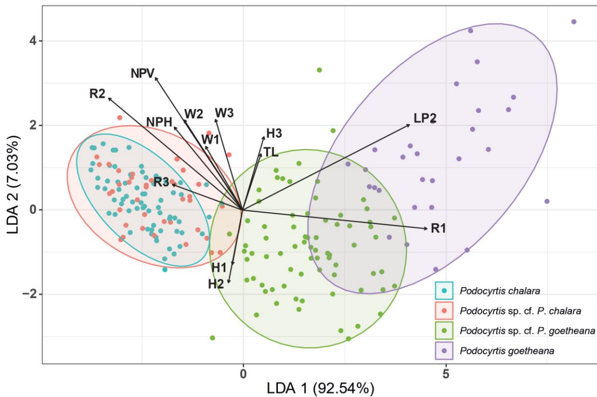
Figure 2. Scatter plot of the two first axes of the Linear Discriminant Analysis (LDA) conducted on the 13 variables that constituted the morphometric data using four a priori identified morphogroups (indicated in the legend; ellipses correspond to the 95 % confidence intervals for each morphogroup). Abbreviations: W1: maximum width of the cephalis without the apical horn; W2: maximum width of the thorax; W3: maximum width of the abdomen; H1: maximum height of the cephalis; H2: maximum height of the thorax; H3: maximum height of the abdomen; TL: total length or height of the specimen without the apical horn; LP2: maximum length of the second abdominal pore; NPV: number of abdominal pores aligned vertically; NPH: number of abdominal pores aligned horizontally; R1: maximum length of the second pore of the abdomen/H3; R2: number of abdominal pores aligned vertically/H3; R3: number of abdominal pores aligned horizontally/W3.
