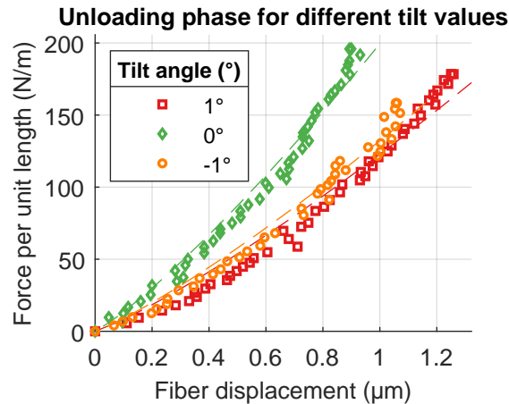
Figure 3.15: Force-displacement results of experimental compression of PA11 fiber for different tilt angles. The data from the simulation is represented with markers which the fitted analytical model represented with dotted lines.
