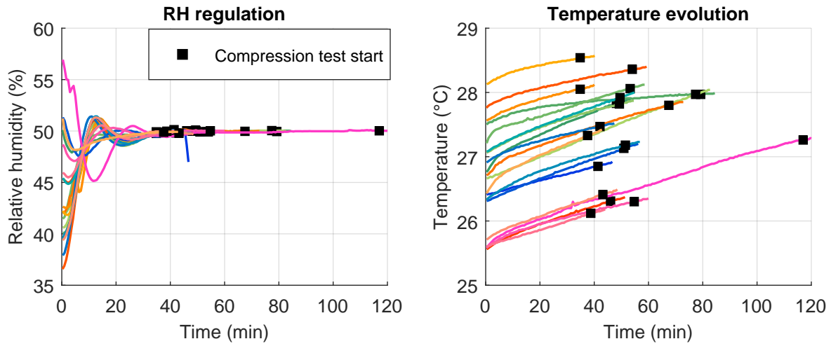
Figure 3.27: Relative humidity regulation and related change in temperature. The start of the compression test is represented with a black square. Each colored line represents a test on a different fiber (Kevlar, flax, hemp or nettle).
