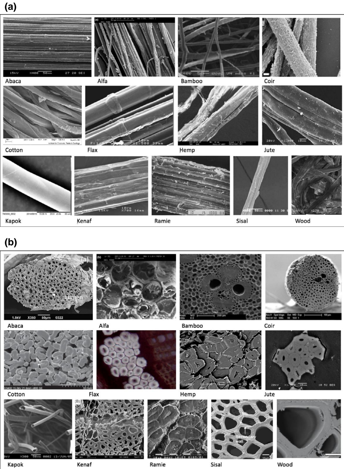
Figure 1.3: SEM images of plant fibers along: (a) the fiber length, (b) the fiber cross section [Bourmaud 18].
