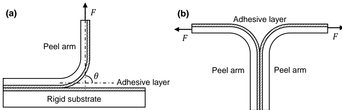
Figure 1.21: (a) Single arm peeling test, (b) T-peeling test. Representation adapted from [Hadavinia 06].
