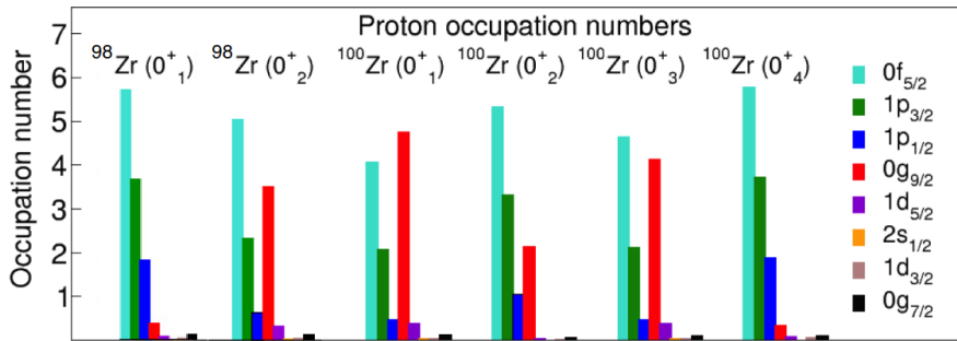
Figure 13.3 – Proton occupation numbers calculated within the MCSM framework for the 0_{1,2}^+ states of ^{98}\text{Zr} and the first four 0^+ states in ^{100}\text{Zr} [183].
