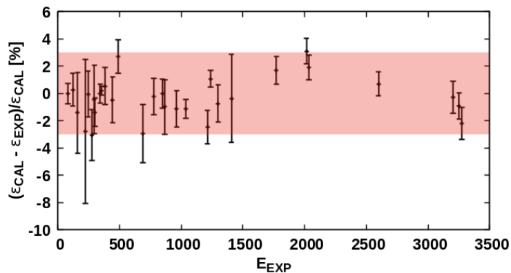
Figure 11.9 – Relative differences in percent between the efficiency \varepsilon_{CAL} calculated using the curve obtained with EFFIT and the experimentally measured values \varepsilon_{EXP} as a function of the energy of the \gamma ray. The shaded area corresponds to the 3% uncertainty adopted in the analysis.
