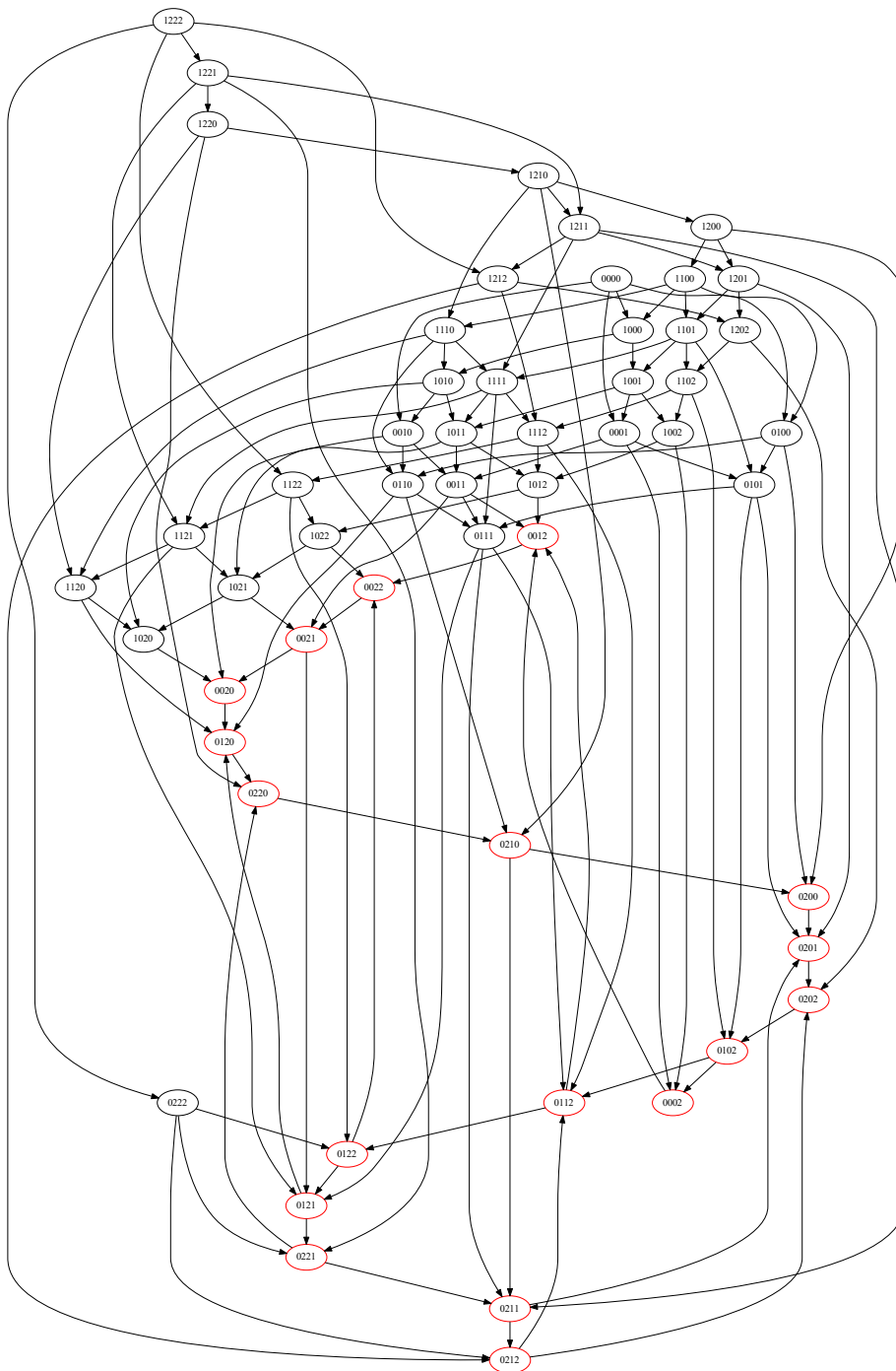
Figure 7.7 – Example of a discrete periodic attractor (red discrete states) that oscillates in 3 dimensions. The discrete model corresponds to the left influence graph in Fig 7.8, with s(G_1 \rightarrow G_0) = s(G_2 \rightarrow G_0) = s(G_3 \rightarrow G_0) = 1 .
