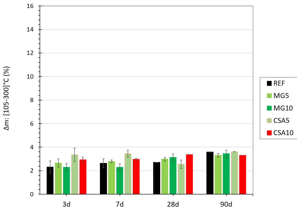
Figure C.1 – Mass loss in the temperature range of [105-300]°C for all the cement-based mortars.
