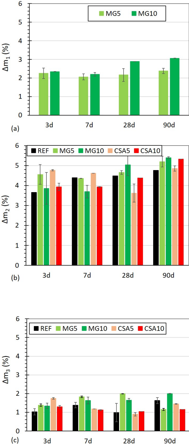
Figure 5.6 – Mass loss in the temperature range equal to [300-450]^{\circ}\text{C} ( \Delta m_1 ) related to brucite (a), [450-600]^{\circ}\text{C} ( \Delta m_2 ) related to portlandite (b) and [600-800]^{\circ}\text{C} ( \Delta m_3 ) related to carbonates-containing phases (c) at 3, 7, 28 and 90 days.
