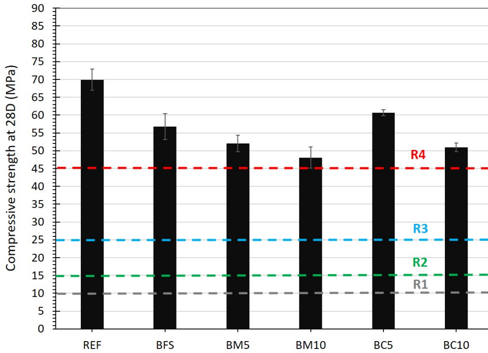
Figure 6.15 – Compressive strength at 28 days for all the studied mortars and the EN 1504-3 standard requirements: non structural (R1 \geq 10 MPa and R2 \geq 15 MPa) and structural (R3 \geq 25 MPa and R4 \geq 45 MPa) element.
