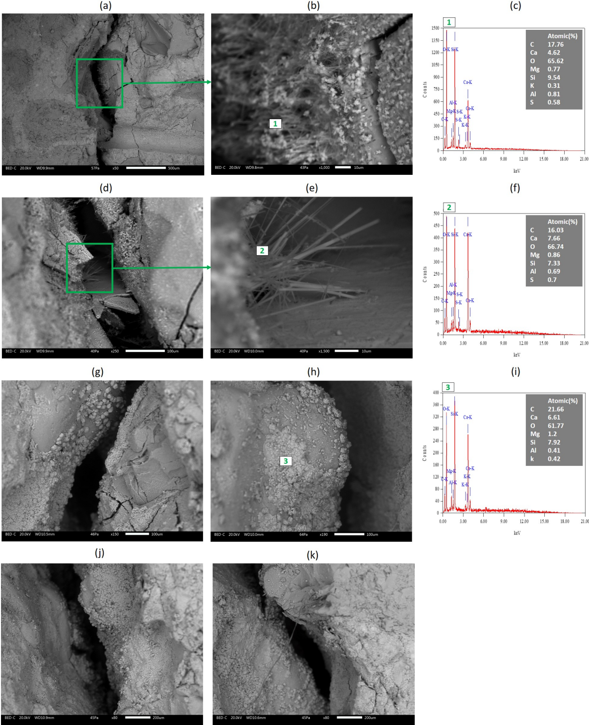
Figure 5.33 – SEM observation of self-healing products inside the crack for MG10 and its EDX analysis.
