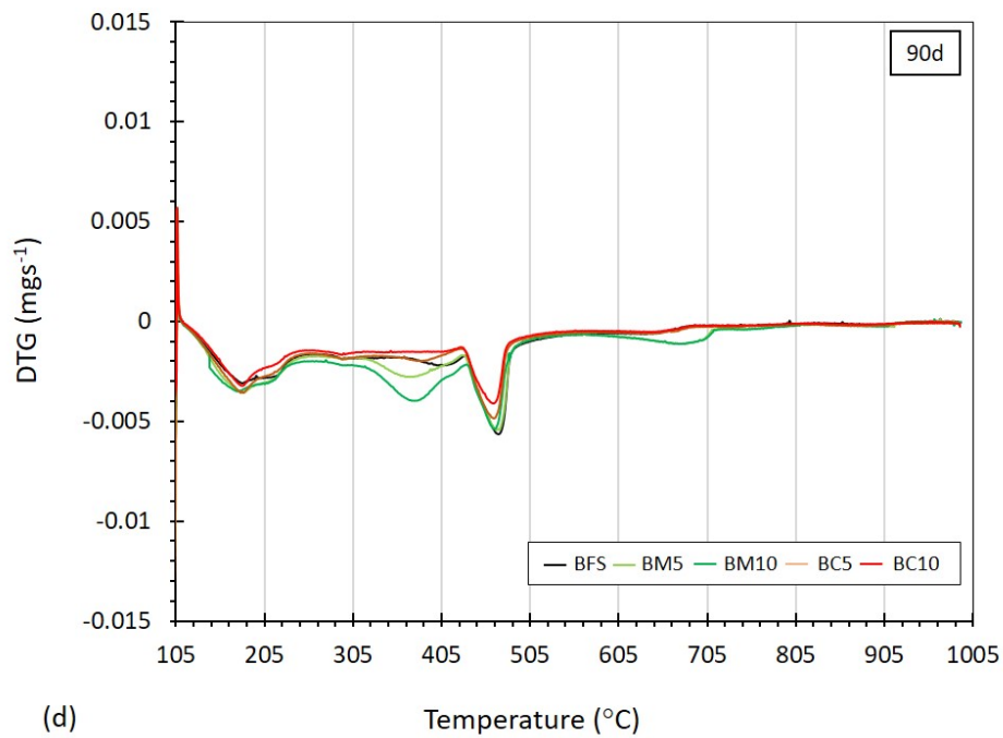
Figure 6.5 – DTG curves of the mixtures at 3 days (a), 7 days (b), 28 days (c) and 90 days (d).
