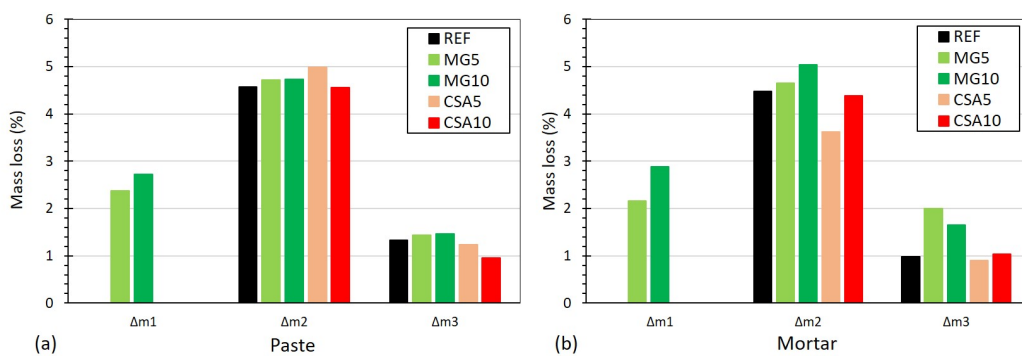
Figure 5.8 – Mass loss at 28 days in the temperature range equal to [300-450]°C ( \Delta m_1 ), [450-600]°C ( \Delta m_2 ) and [600-800]°C ( \Delta m_3 ) for paste mixtures (a) and mortar mixtures (b).
