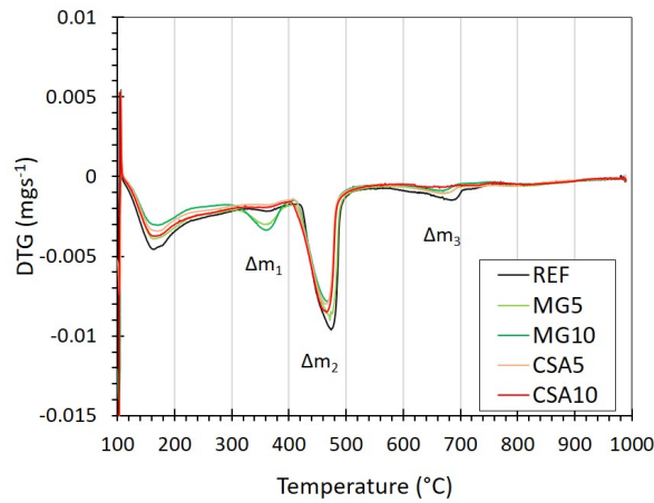
Figure 5.7 – DTG curves for paste mixtures at 28 days.
