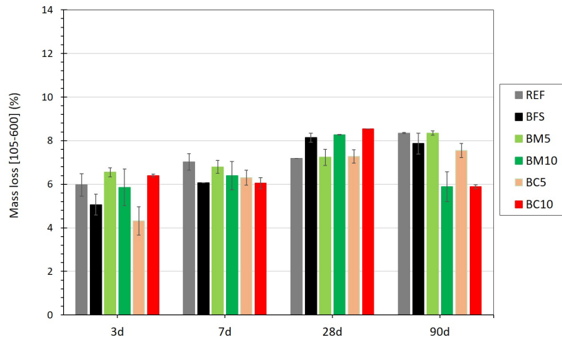
Figure D.2 – Mass loss in the temperature range of [105-600]°C for all the blended mortars.
