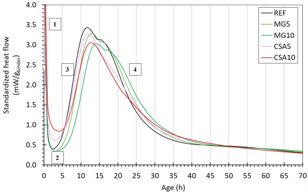
Figure 5.1 – Standardized heat flow for all the studied mixtures; (1) Pre-induction period; (2) Dormant period; (3) Acceleration period and (4) Post-acceleration period; and its cumulative heat (b).
