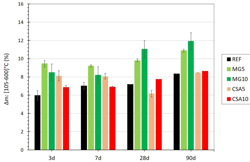
Figure C.2 – Mass loss in the temperature range of [105-600]°C for all the cement-based mortars.
