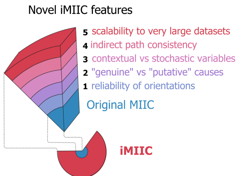
FIGURE 2.9 – MIIC interprétable (iMIIC).
