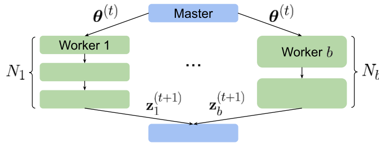
Figure 2.1 – Illustration of one global iteration of Algorithm 2.1 . For each worker, the width of the green box represents the amount of time required to perform one LMC step.
