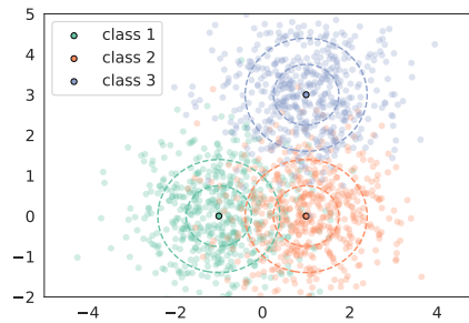
Figure 5.4 – Simulated data distribution: 3 two-dimensional Gaussians with means \theta_1 = [-1, 0] , \theta_2 = [1, 0] , \theta_3 = [1, 3] and identity covariance matrices.
