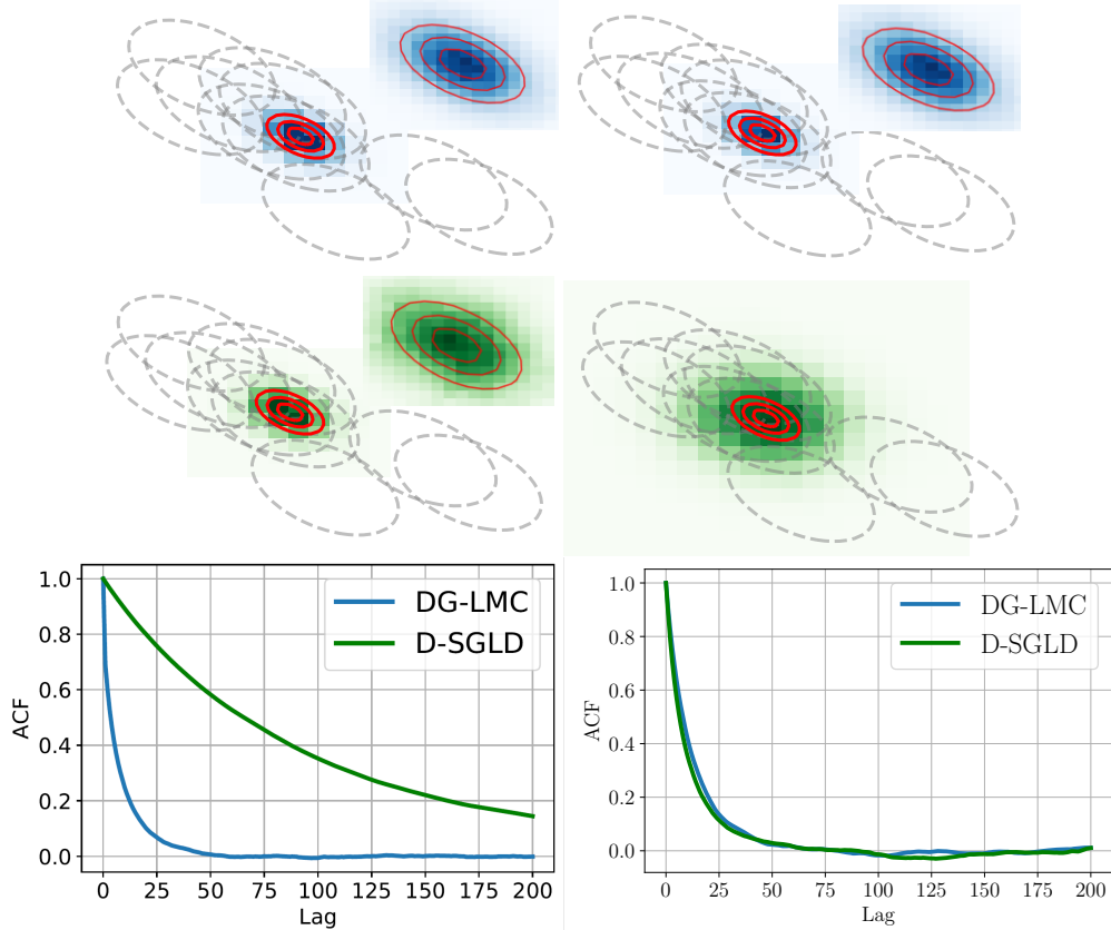
Figure 2.2 – Toy Gaussian experiment. (left) N = 1 local iterations and (right) N = 10 . (top) DG-LMC, (middle) D-SGLD and (bottom) ACF comparison between DG-LMC and D-SGLD.
