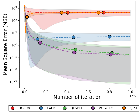
Figure 3.2 – MSE comparison with p_c = 1/5 and \gamma = \bar{\gamma}/3 .
