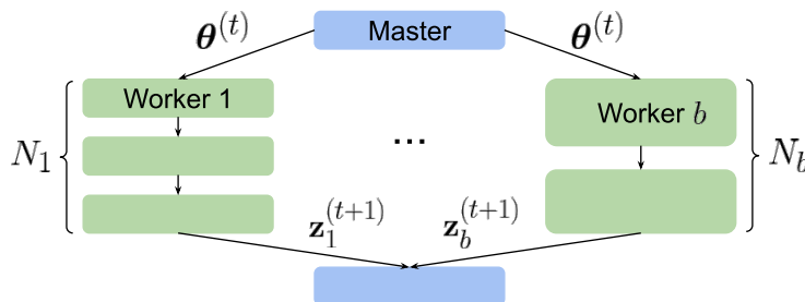
Figure 2.1 – Illustration of one global iteration of Algorithm 2.1 . For each worker, the width of the green box represents the amount of time required to perform one LMC step.
