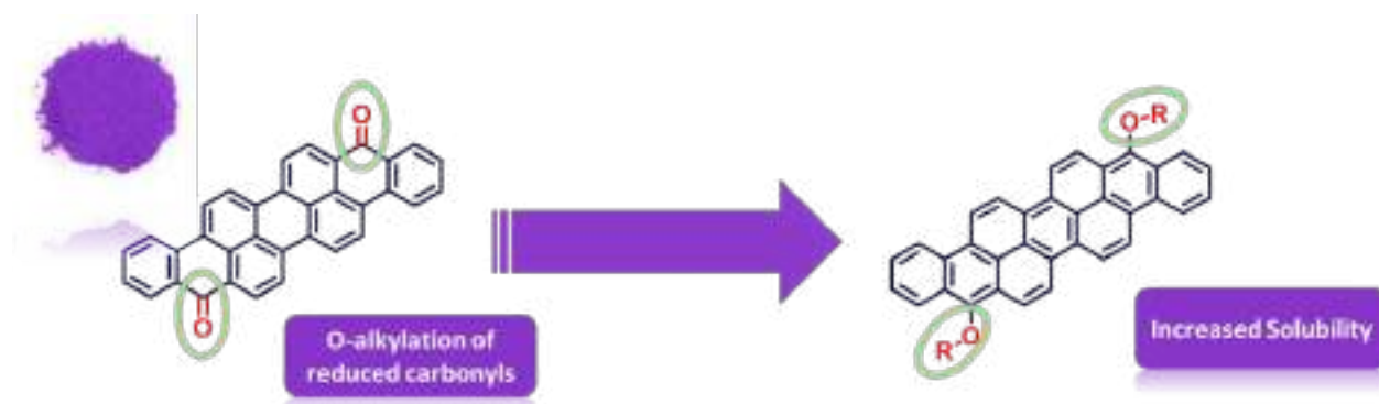
Figure 3.33 Structure of the Isoviolanthrone vat dye and potential target O-alkylated “soluble” compounds.
