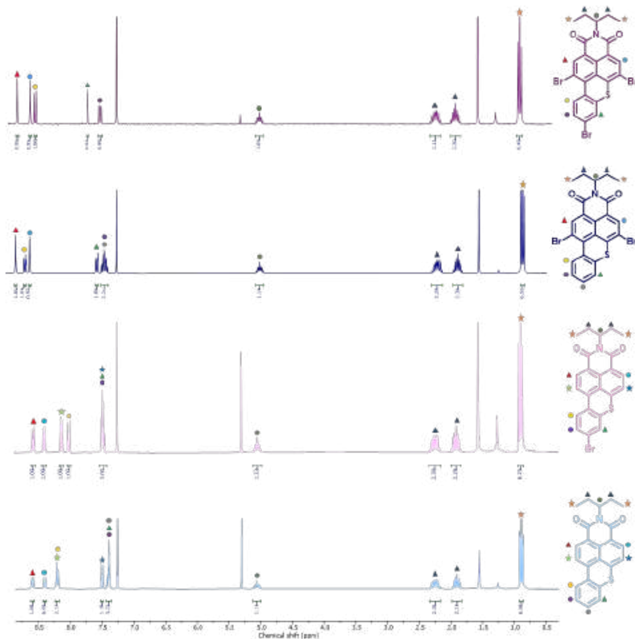
Figure 3.25 300 MHz NMR spectra of BTI , BTI-N-Br , BTI-Br 2 , and BTI-Br 3 in CDCl 3 with signals attributions.
