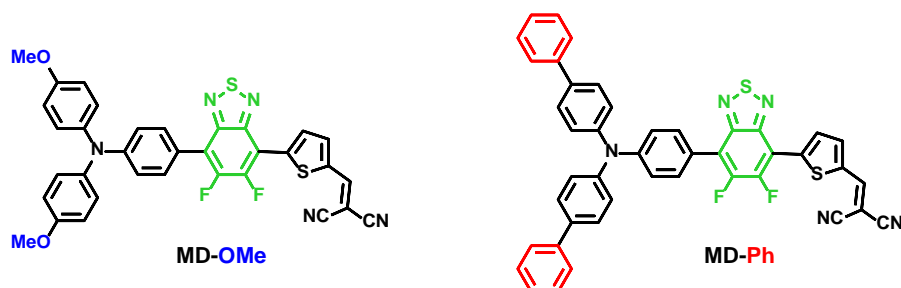
Figure 2.11 Chemical structures of the target push-pull derivatives.
