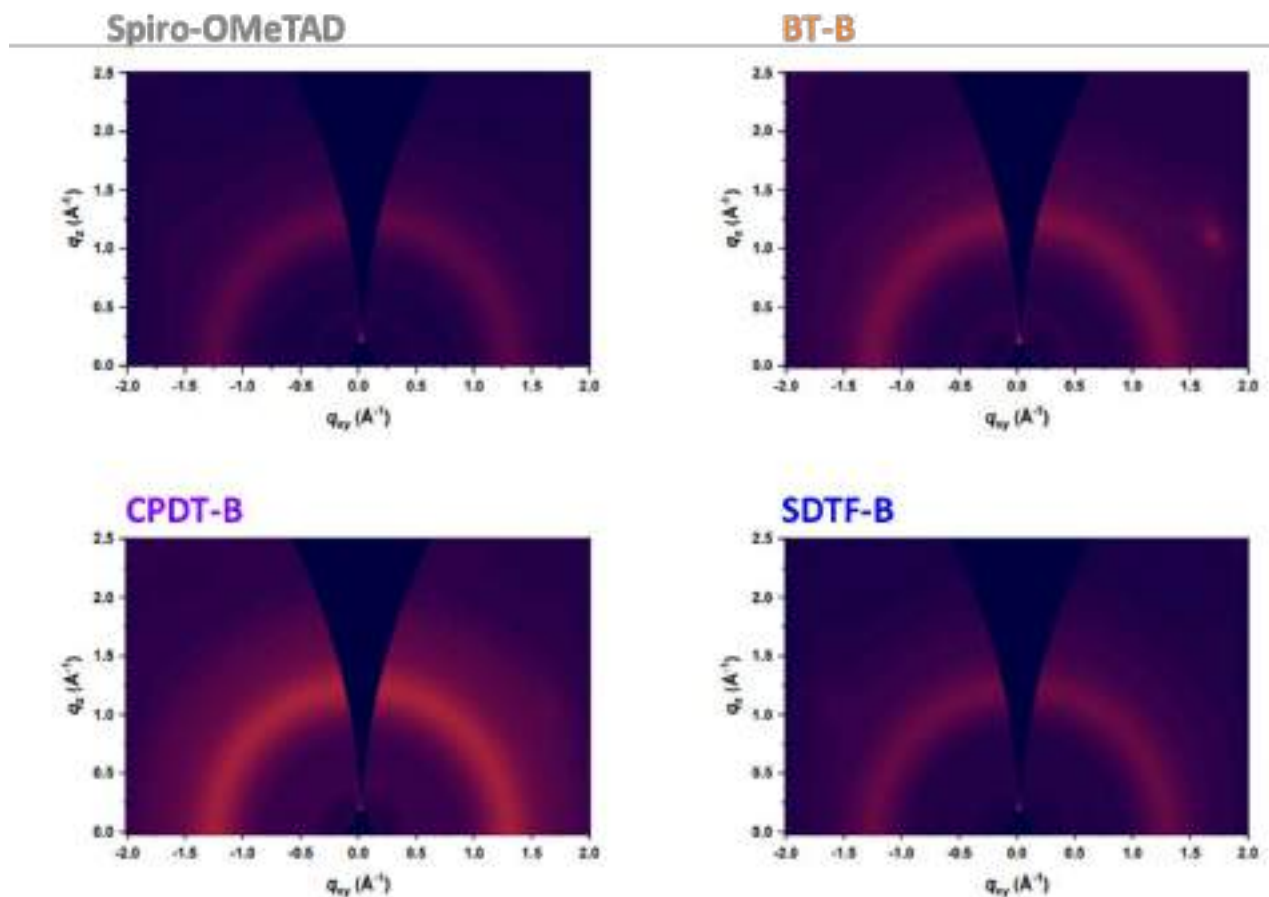
Figure 2.42 Grazing incidence wide angle X-ray scattering (GIWAXS) patterns of as-prepared pristine spiro-OMeTAD and blends. The samples were prepared on silicon substrate and dopants were added.
