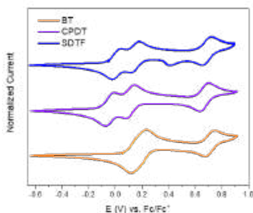
Figure 2.32 Cyclic voltammograms of BT , CPDT , and SDTF molecules, 1 mM in 0.1 M TBAPF 6 in CH 2 Cl 2 with a scan rate of 100 mV/s.
