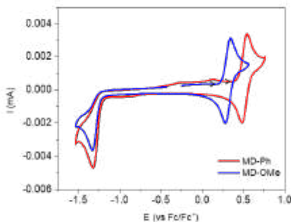
Figure 2.12 Cyclic voltammograms of MD-OMe and MD-Ph molecules, 0.5 M in 0.1 M \text{TBAPF}_6 in \text{CH}_2\text{Cl}_2 with a scan rate of 100 mV/s.
