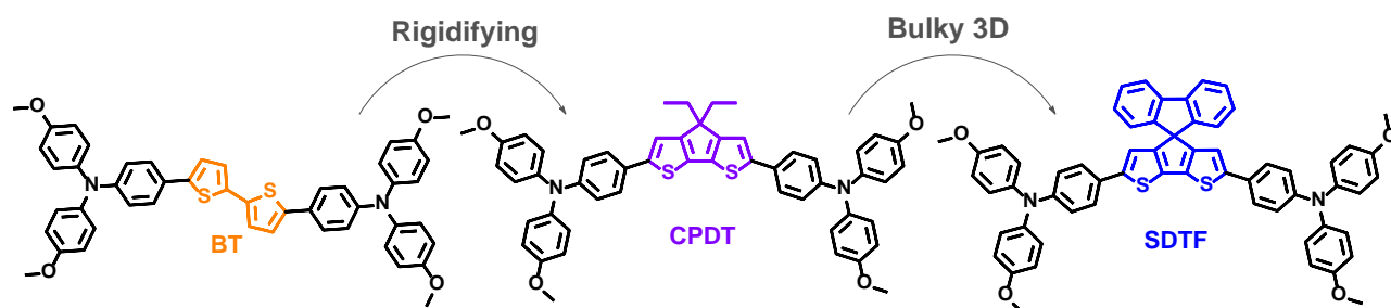
Figure 2.31 Structures of the three target HTMs.
