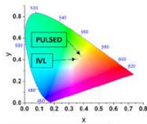
Figure 3.39 CIE chromaticity diagram of the DBP LEC device under IVL and pulse current mode.
