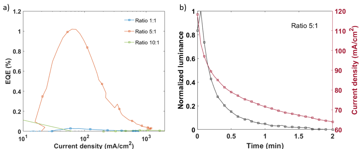
Figure III.23. a) Correlation of EQE and current density and b) Device durability in PeLEDs based on perovskite QD/PEO composites.
