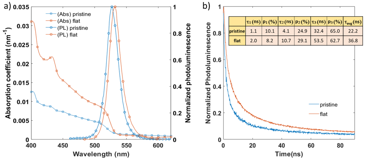
Figure IV.8. Comparison of optical properties between non-imprinted and flat-imprinted perovskite films on PEDOT:PSS-coated glass substrates: a) UV-Vis absorption coefficients and PL spectra and b) Time-resolved PL decay. The inset shows the fitting parameters of the samples' PL lifetime using the tri-exponential model.
