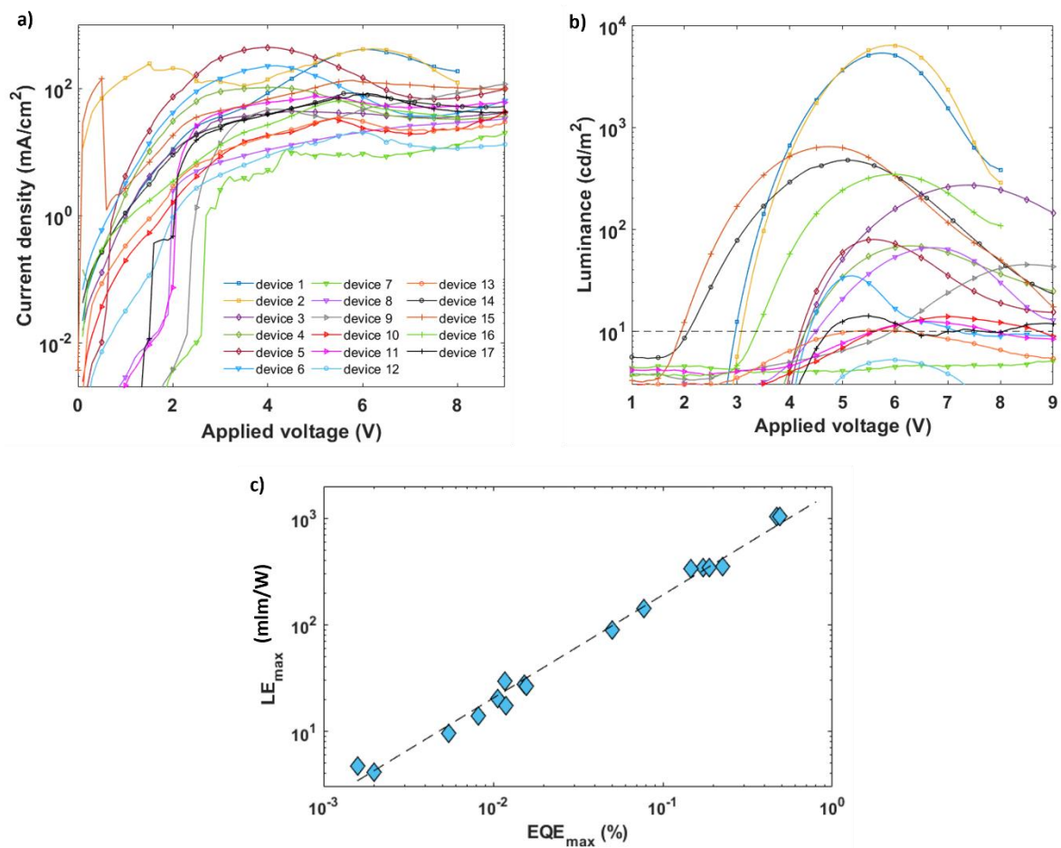
Figure II.12. Low reproducibility in a set of 17 quasi-2D PeLEDs: a) J-V curves, b) L-V curves. The dotted line indicates the threshold luminance of 10 \text{cd/m}^2 , and c) statistics of maximum EQE and LE values. The straight line represents the linear relation between the two quantities.
