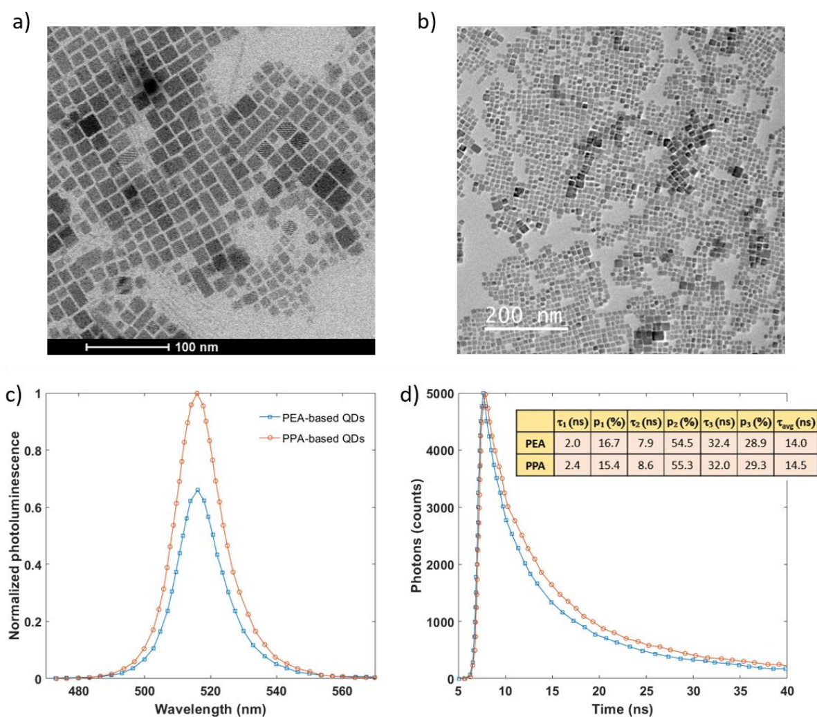
Figure III.2. TEM images of CsPbBr 3 QDs synthesized with PPA at scale bars of a) 100 nm and b) 200 nm, respectively; and Comparison of optical properties of CsPbBr 3 QDs synthesized with PEA and PPA: c) steady-state PL emission and d) PL lifetime (The inset shows the fitting parameters and estimated average lifetime). The data is provided by C. Mayer.
