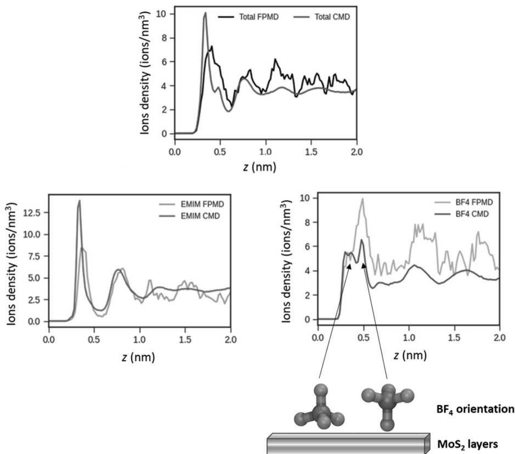
Figure 4.17. EMIM- \text{BF}_4 ions COM density profiles with respect to the distance from the \text{MoS}_2 pristine surface obtained by FPMD at 300K ( z=0 at the position of S atoms of the top layer of the top \text{MoS}_2 ). Top: total density profiles. Bottom: Density profiles of EMIM (left) and \text{BF}_4 (right) ions. For comparison, the density profiles obtained by classical MD at 300K are also shown.
