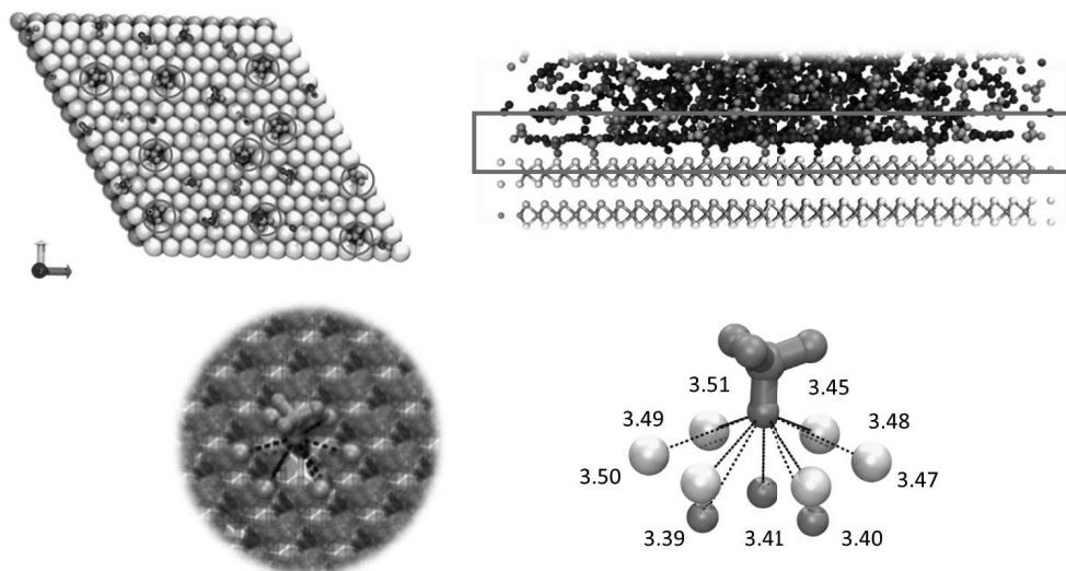
Figure 4.10. Top (left) and lateral (right) views of the saturation of the surface S vacancies by BF 4 ions for the MoS 2 model with a surface defect density of 4.0 \times 10^{14} sites/cm 2 . In the top view, the locations of the defect sites are highlighted with a orange circle. Bottom: (left) typical configuration of a BF 4 ion that is located on top of a S surface vacancy and (right) a model where the F...Mo and F...S interatomic distances are reported in Å. Color legend: EMIM ions in blue; BF 4 in orange; S atoms in yellow and Mo atoms in cyan.
