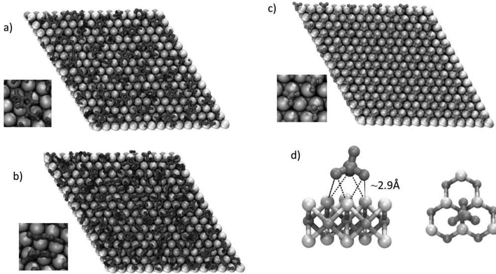
Figure 5.5. Snapshots of EMIM and BF 4 ions orientation within the first interfacial layer obtained in the following charged models: majority of EMIM ions lying parallel (a) and perpendicular (b) to the MoS 2 charged surfaces at 3 \mu\text{C}/\text{cm}^2 and 73 \mu\text{C}/\text{cm}^2 ; c) BF 4 ions structured orientation found with 73 \mu\text{C}/\text{cm}^2 surface charge. We show the well organized orientation of BF 4 ions with three F atoms closely interacting with three S atom so the MoS 2 surface.
