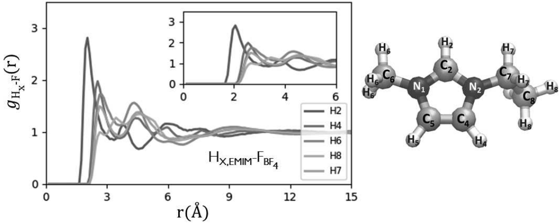
Figure 3.6. Left panel: Pair correlation functions g_{ij}(r) of the different H atoms of \text{EMIM}^+ with the F atoms of \text{BF}_4^- obtained by classical MD at room temperature. Inset: a zoom-in in the 1-6Å region. Right panel: The atom numbering is the standard one given in the literature and reported explicitly here.
