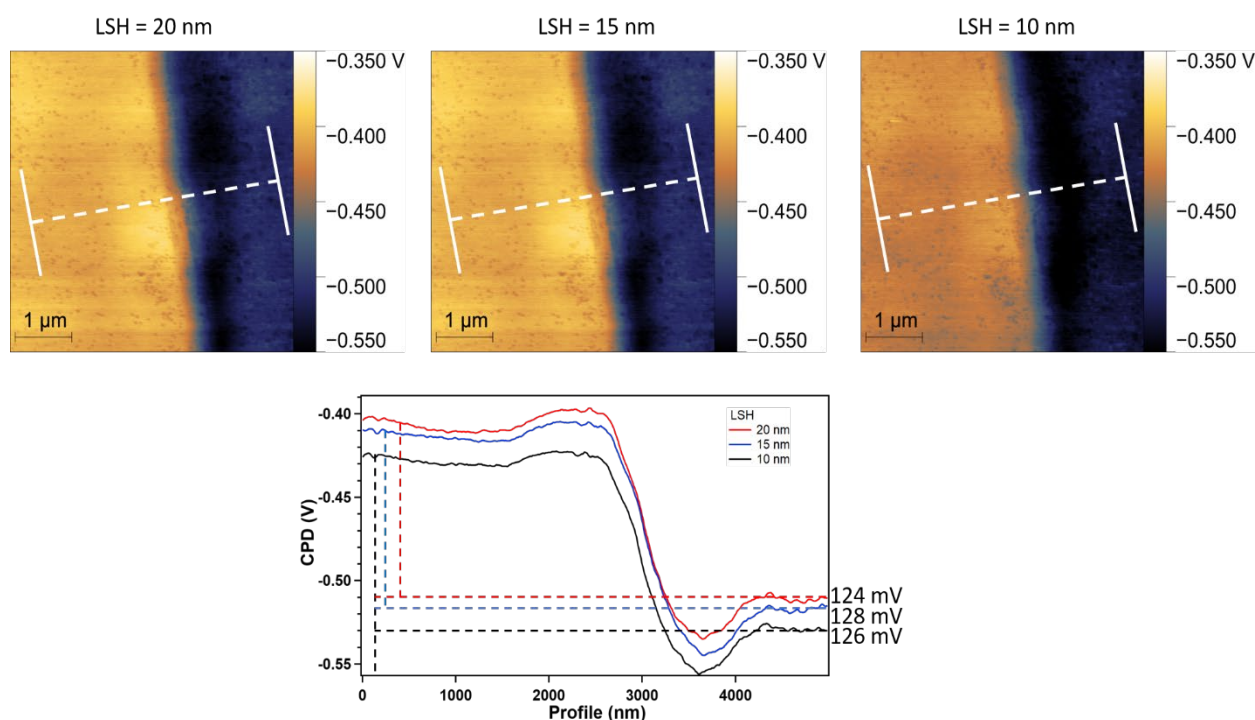
Figure S17. Variation of the CPD as a function of the LSH. At the top are shown CPD images of the same area (5 μm 2 ) of an AfFtn-AA 4800Fe monolayer sample, at different LSH = 20 nm (left), LSH = 15 nm (center), and LSH = 10 nm (right). At the bottom are shown CPD profiles taken from the CPD images (from the white dashed line) across the ferritin monolayer silicon intersection. The values of the ferritin CPD compared to the silicon CPD are shown to the right of the graphic for each LSH value.
