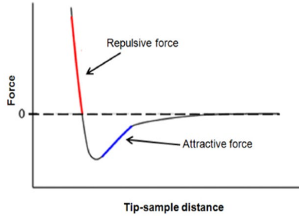
Figure 43 : A typical inter-atomic force vs. distance curve. The force gradient (a derivative of the curve) is limited to the short-range in tip-sample distance, while the force is long-ranged compared to the force gradient. [139]
