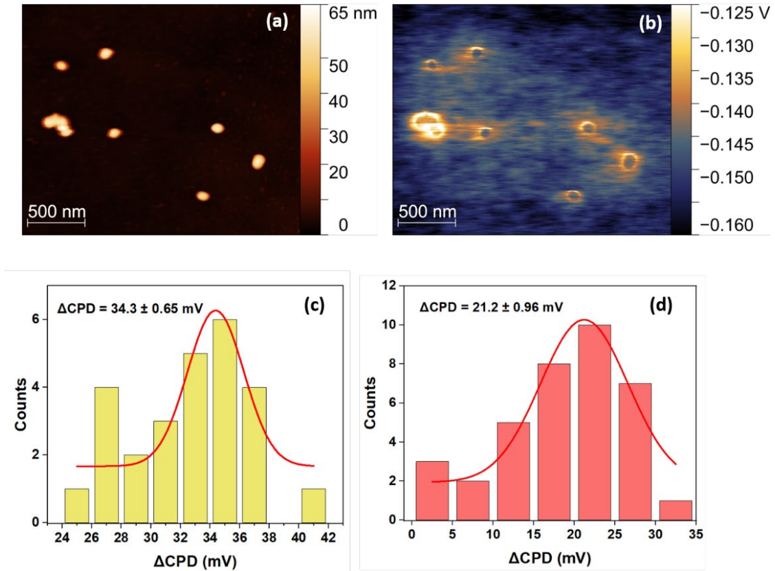
Figure 53: KPFM topography (a) and CPD (b) images of gold nanoparticles on p -doped silicon wafer ( N_D = 10^{14} - 10^{15} \text{ cm}^{-3} ). Distributions of \Delta\text{CPD} measured for gold nanoparticles on n -doped (c) and p doped (d) silicon substrates. In both cases, the dopant concentration was 10^{15} \text{ cm}^{-3} ( 10\text{-}20 \text{ } \Omega.\text{cm} ).
