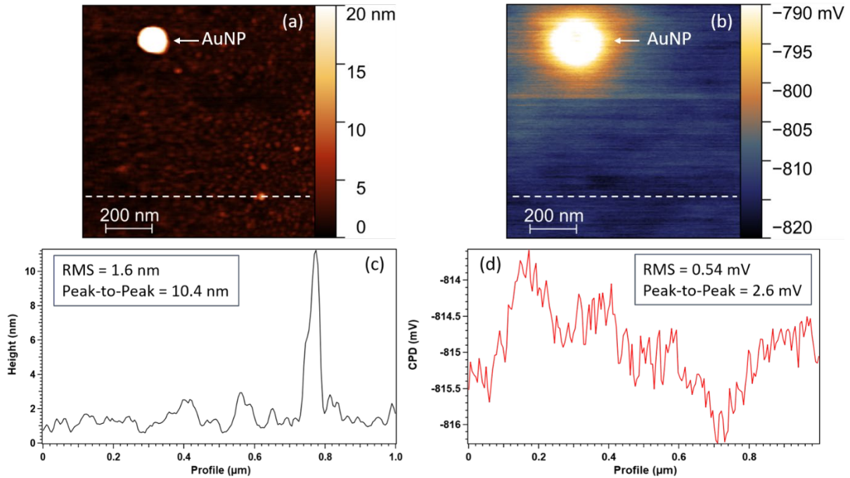
Figure S10: Topography image (a) and its corresponding CPD image (b) of one gold nanoparticle on n -doped silicon (sample A). Profiles (from the white dashed line) below show the height (c) and CPD (d) of a part of the APTES monolayer. Root Mean Square (RMS) and Peak-to-Peak values along these lines are displayed in the inset of the graphs.
