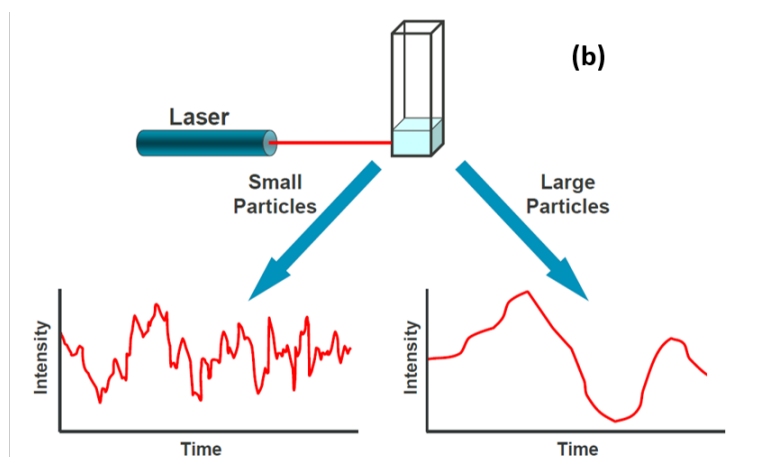
Figure 32 : (a) Schematic of the hydrodynamic diameter of a particle in ionic solution. (b) DLS measurement principle. [127]
