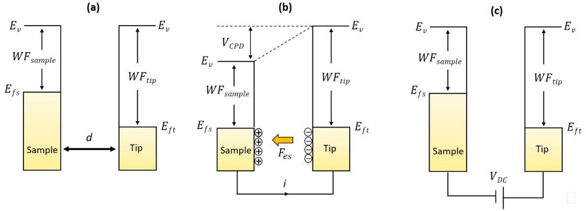
Figure 42: Electronic energy levels of the sample and AFM tip in three cases: (a) tip and sample are separated by a distance d with no electrical contact; (b) tip and sample are in electrical contact; and (c) external bias ( V_{DC} ) is applied between tip and sample to nullify the CPD and, therefore, the tip-sample electrical force. E_v is the vacuum energy level. E_{fs} and E_{ft} are Fermi energy levels of the sample and tip, respectively. [139]
