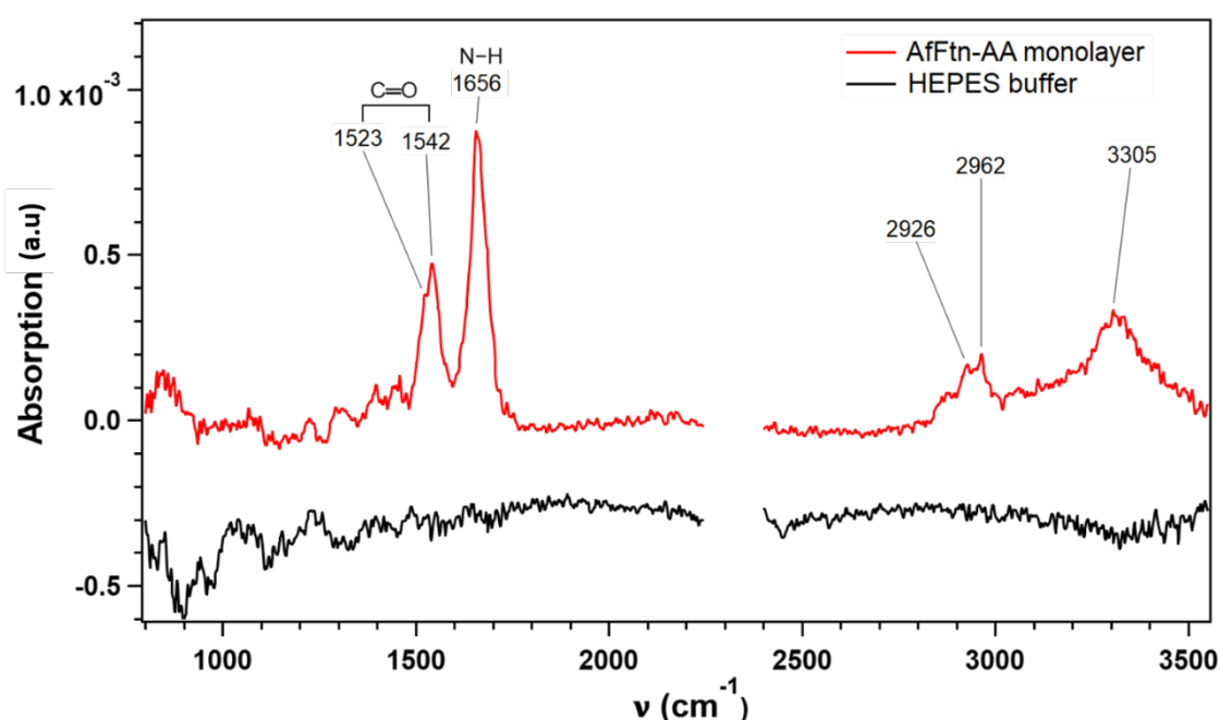
Figure 59: Differential FTIR spectrum (3500–800 \text{cm}^{-1} ) of a ferritin (AfFtn-AA 4800Fe) monolayer (red curve) and HEPES buffer (black curve) on a silicon wafer (FZ). The blank space at 2250-2400 \text{cm}^{-1} corresponded to the \text{CO}_2 vibration peaks that were erased on both curves for the sake of clarity.
