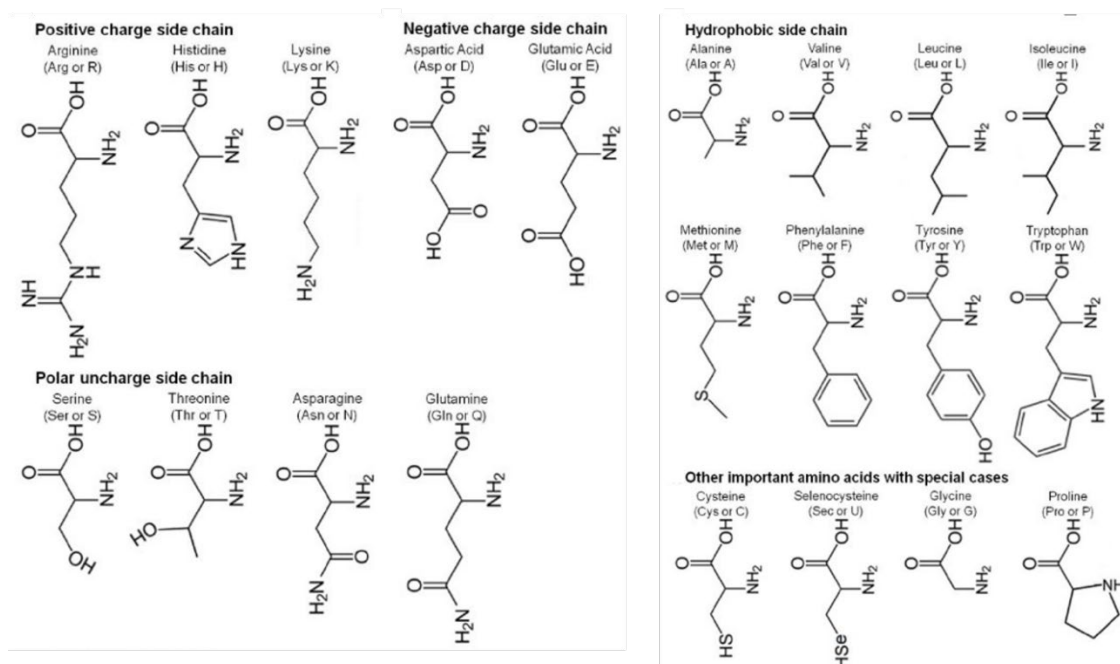
Figure S1 : The 21 amino acid molecules. Each amino-acid is designated with either one letter (e.g., R for Arginine) or the three first letters of its name (e.g., Arg for Arginine).
