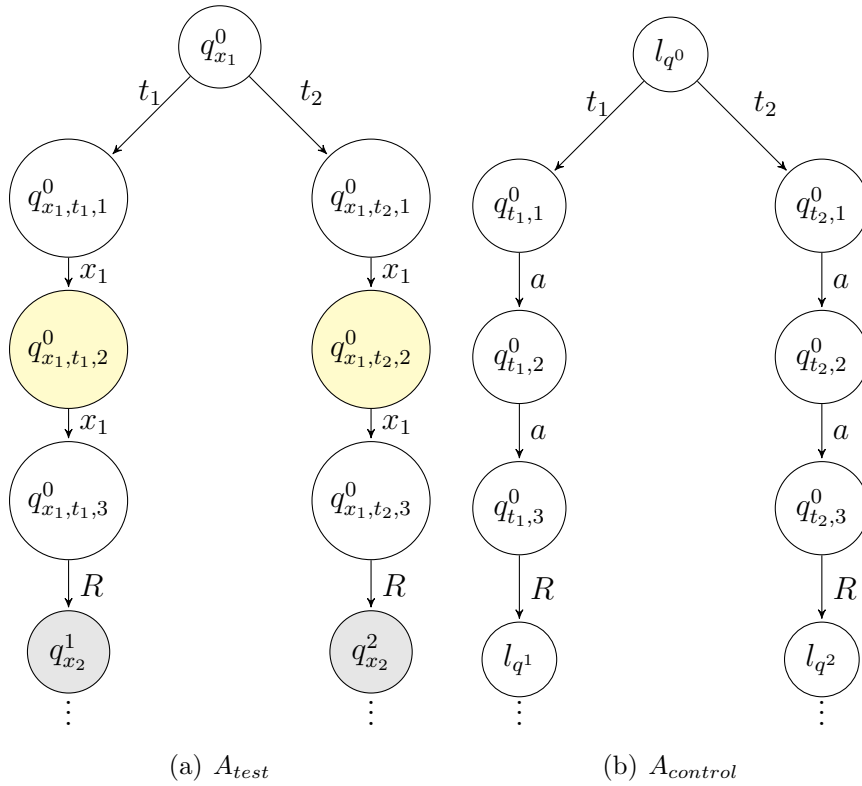
Figure 5.8: Example of Universal Construction Corresponding to q_0
