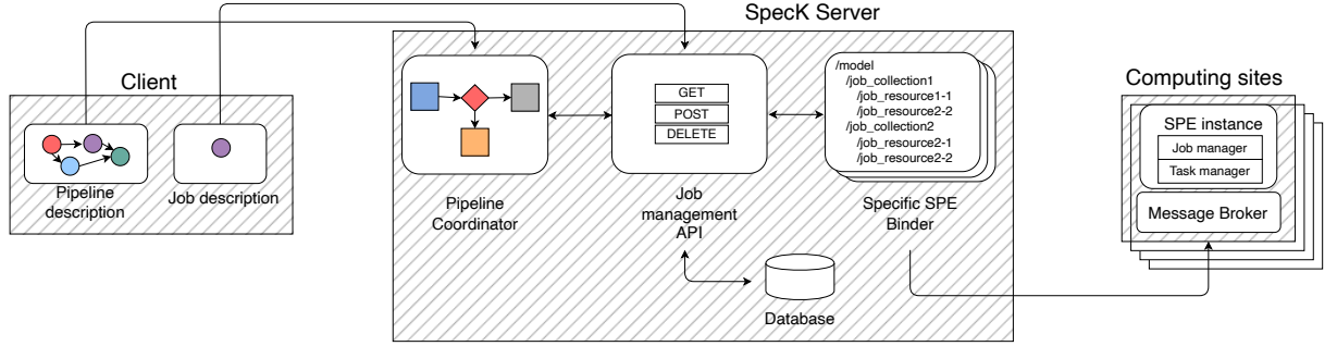
Figure 3.5 – SpecK software architecture.
