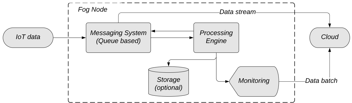
Figure 5.2 – The FogGuru platform software architecture.
