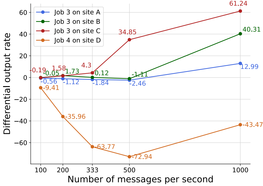
Figure 3.11 – Differential output rate.
